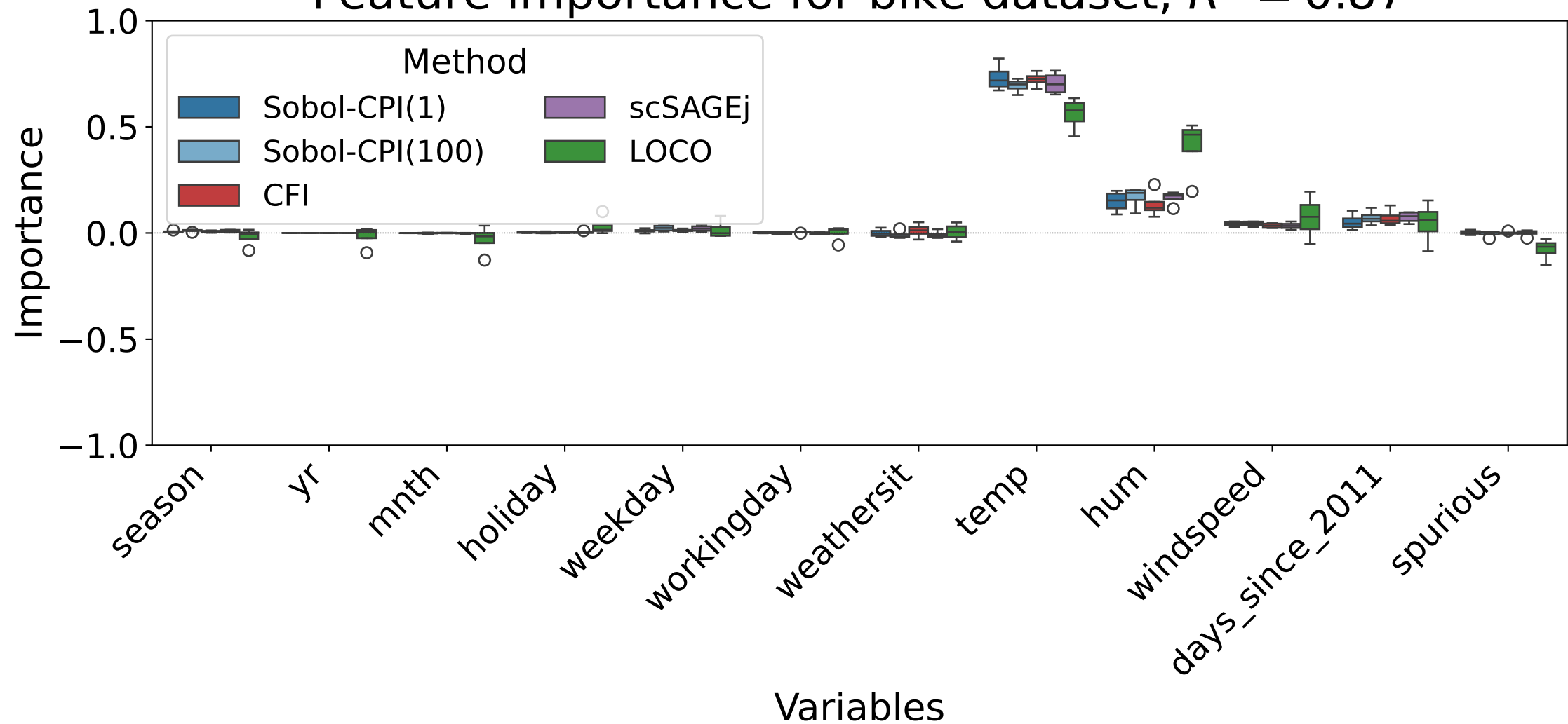
Feature importance for bike dataset, R^2 = 0.87
