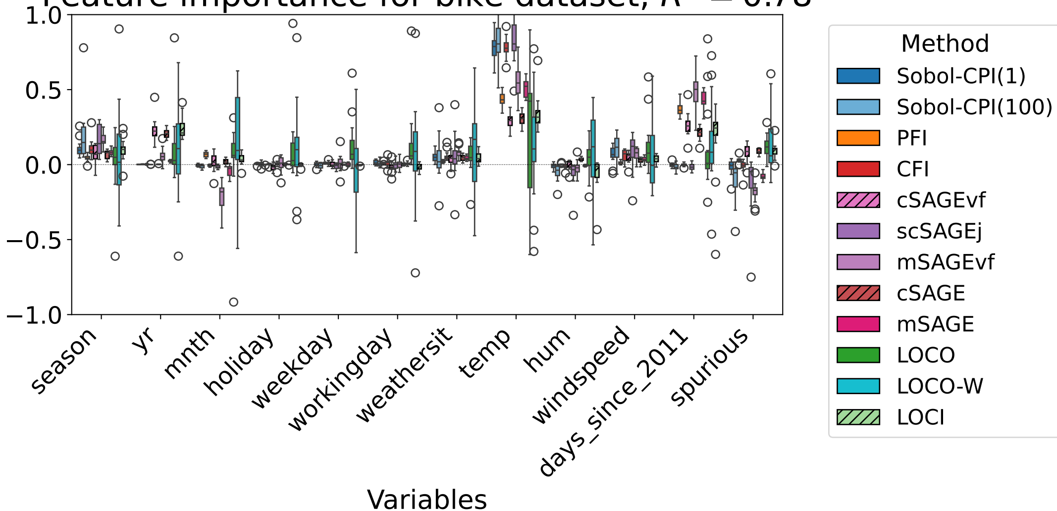
Feature importance for bike dataset, R^2 = 0.78
