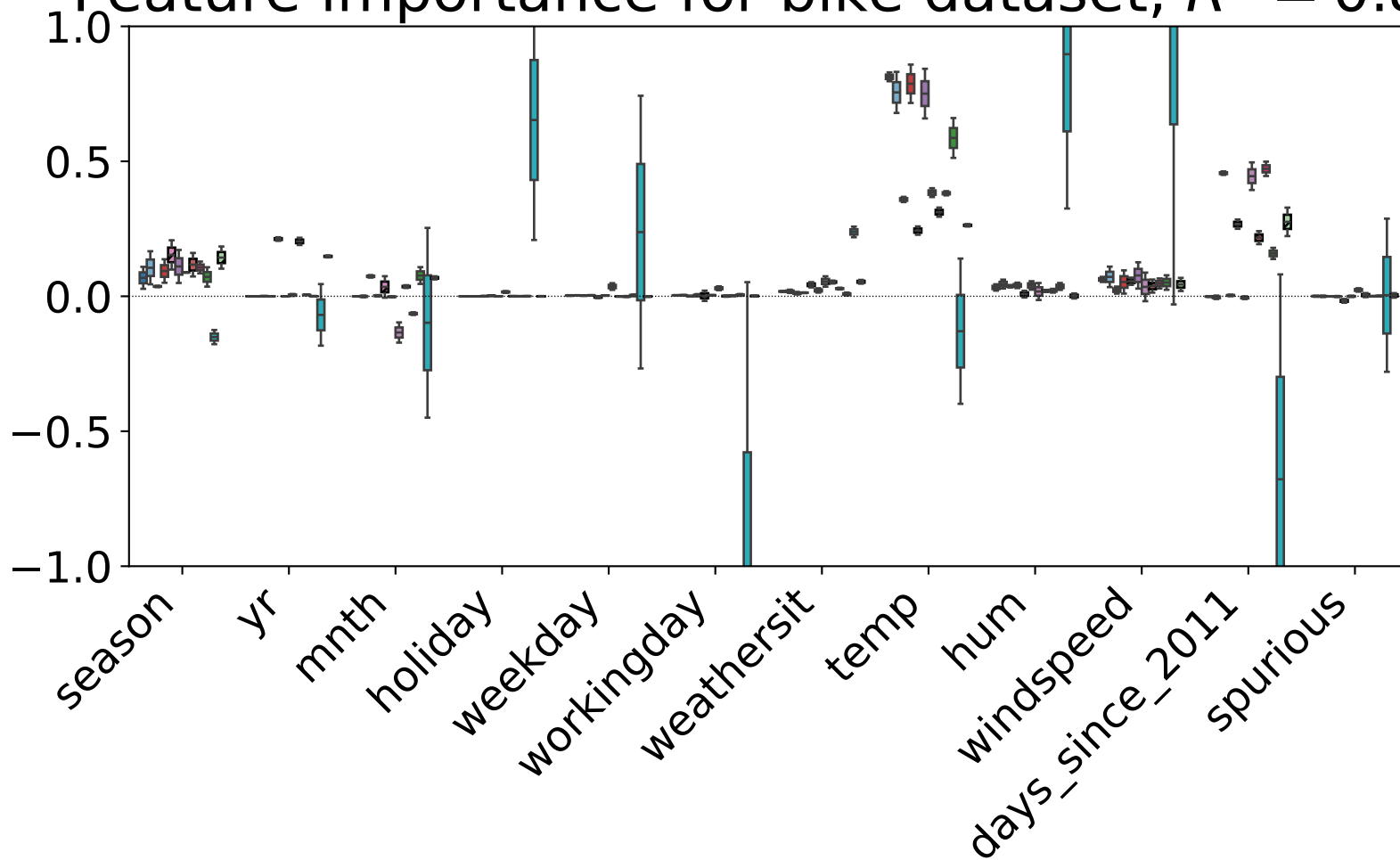
Feature importance for bike dataset, R^2 = 0.80
