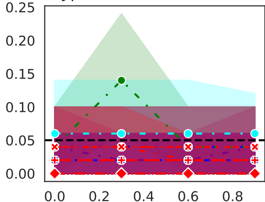
Type-I Error (null feature)
