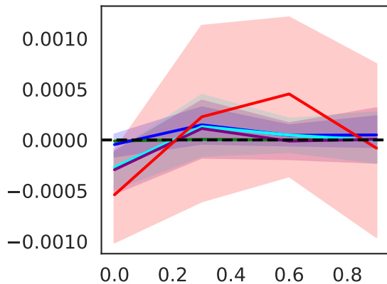
Type-I Error (null feature)
