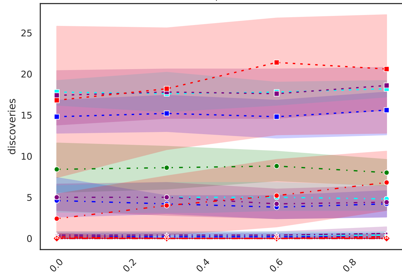
Discoveries (p-value &lt; 0.05)
