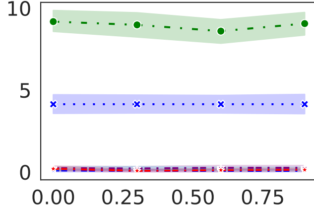
Discoveries ( p < 0.05 )
