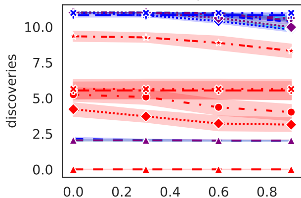
Discoveries ( p < 0.05 )
