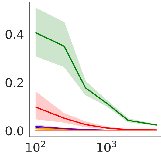
Bias null
