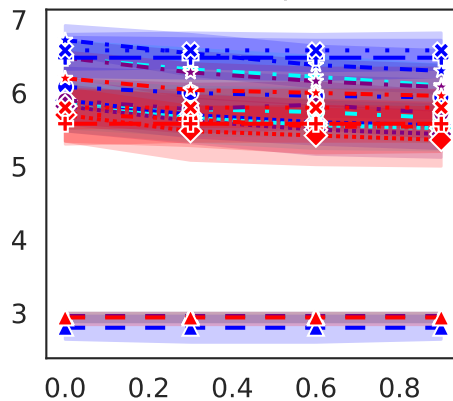
Discoveries ( p < 0.05 )
