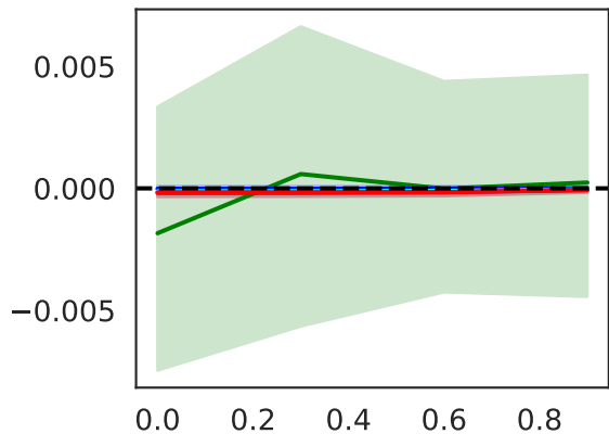
Type-I Error (null feature)
