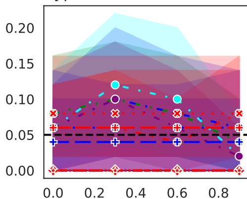
Type-I Error (null feature)
