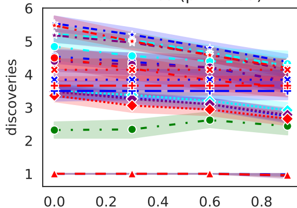
Discoveries ( p < 0.05 )
