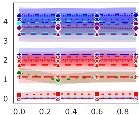
Discoveries ( p < 0.05 )
