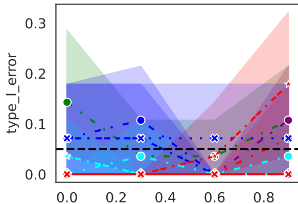
Type-I Error (null feature)
