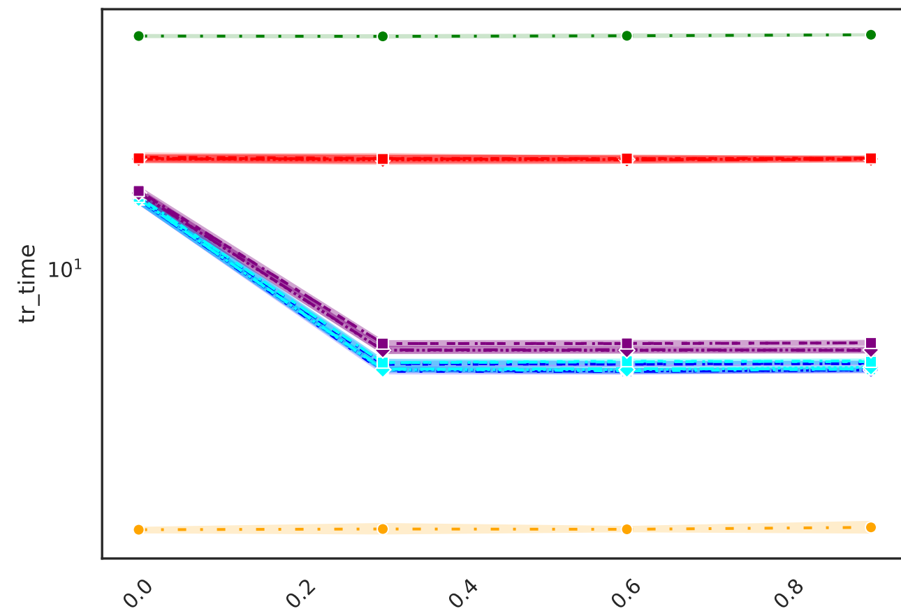
Execution time
