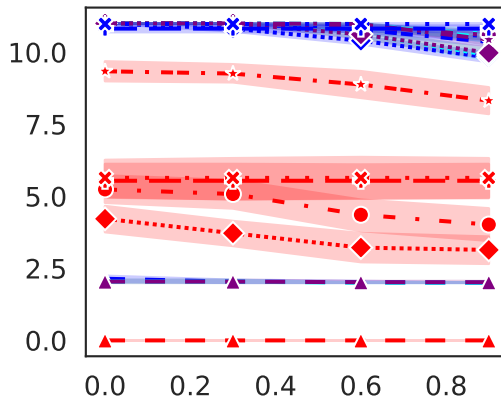
Discoveries ( p < 0.05 )
