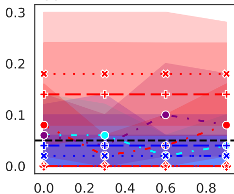
Type-I Error (null feature)
