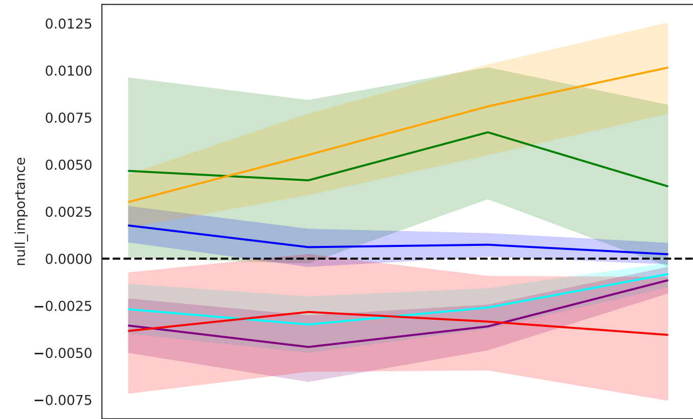
Importance of artificial null feature
