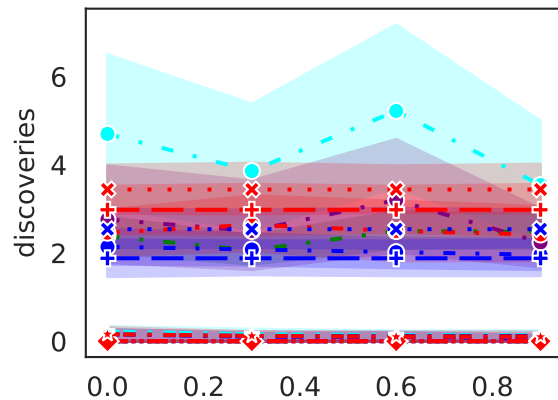
Discoveries ( p < 0.05 )
