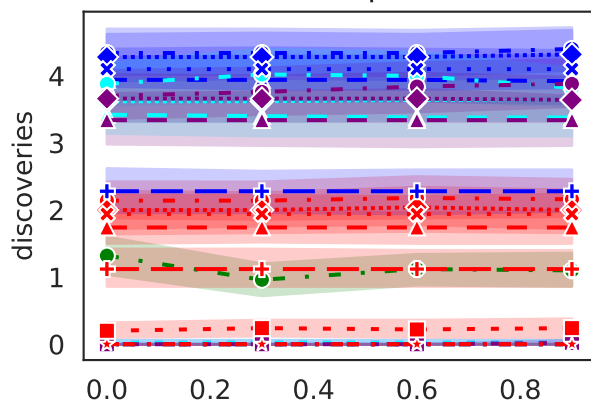
Discoveries ( p < 0.05 )
