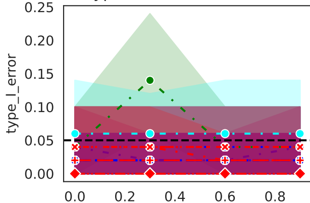
Type-I Error (null feature)
