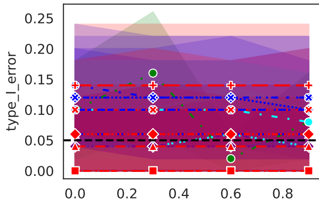
Type-I Error (null feature)
