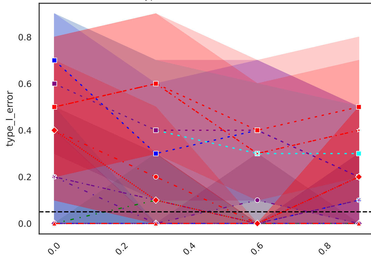
Type-I Error (on null feature)
