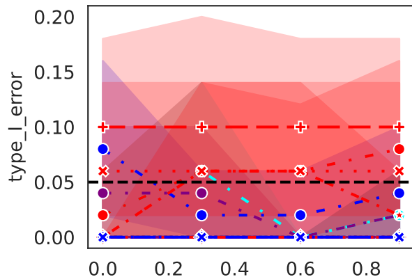
Type-I Error (null feature)
