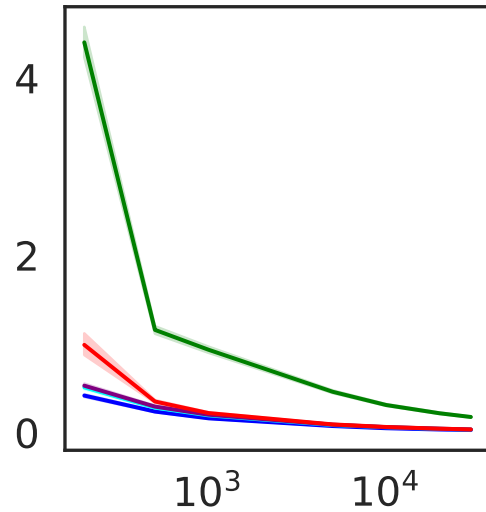
Bias non-null
