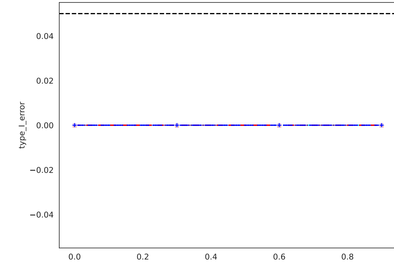
Type-I Error (null feature)
