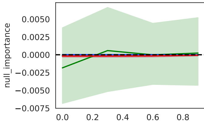
Importance of artificial null feature
