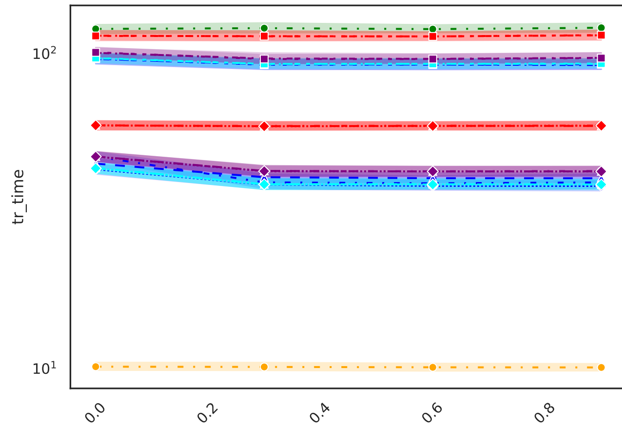
Execution time
