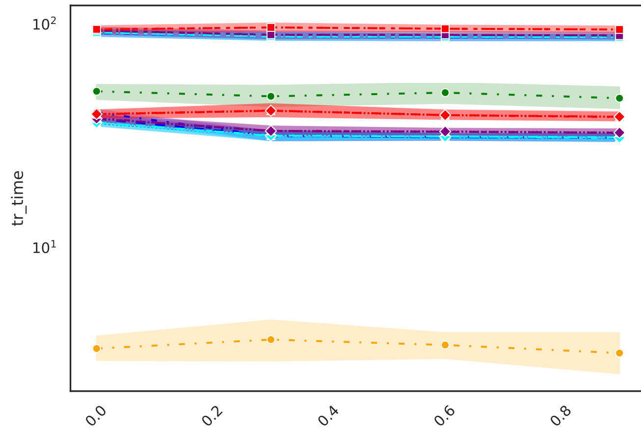
Execution time
