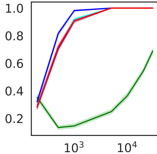
Power
