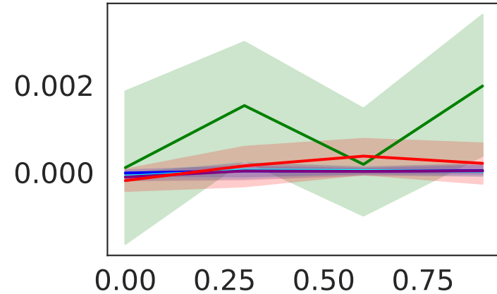
Null Importance
