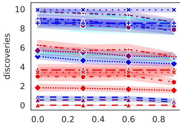
Discoveries ( p < 0.05 )
