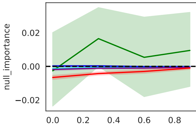
Importance of artificial null feature
