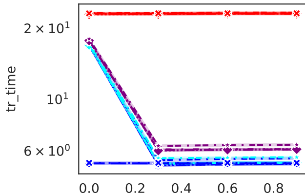
Execution time (log scale)
