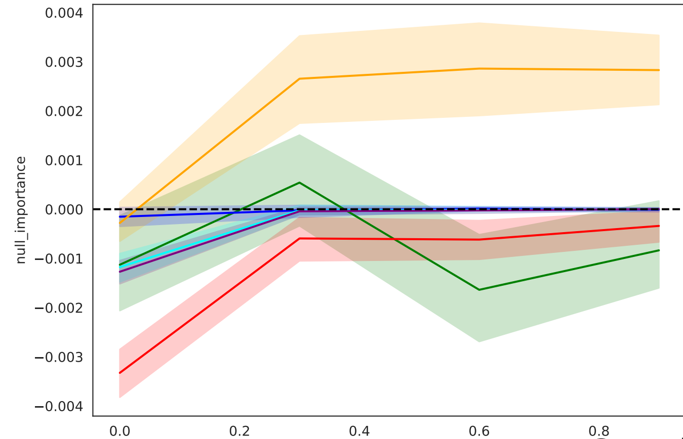
Importance of artificial null feature
