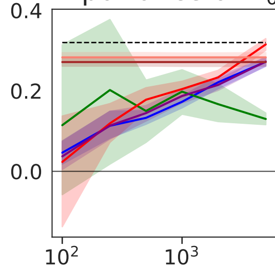
Importance of X_0
