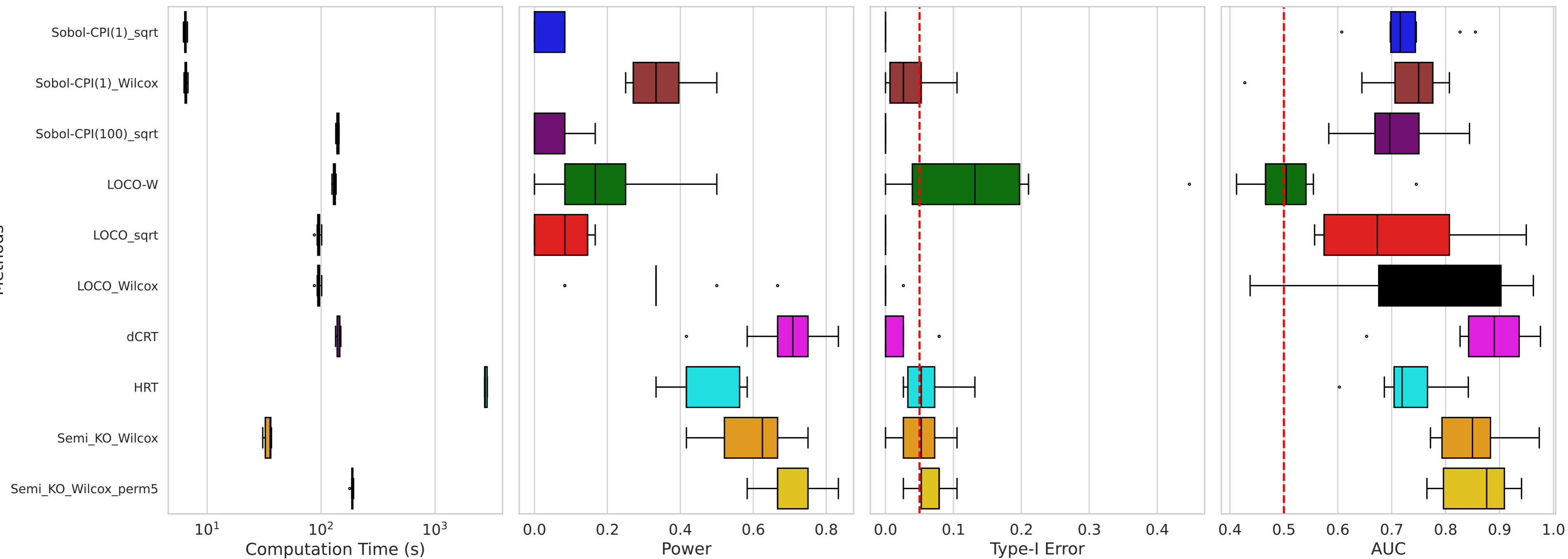
Inference Results (R2 HRT=0.596, R2 Semi_KO=0.632)
