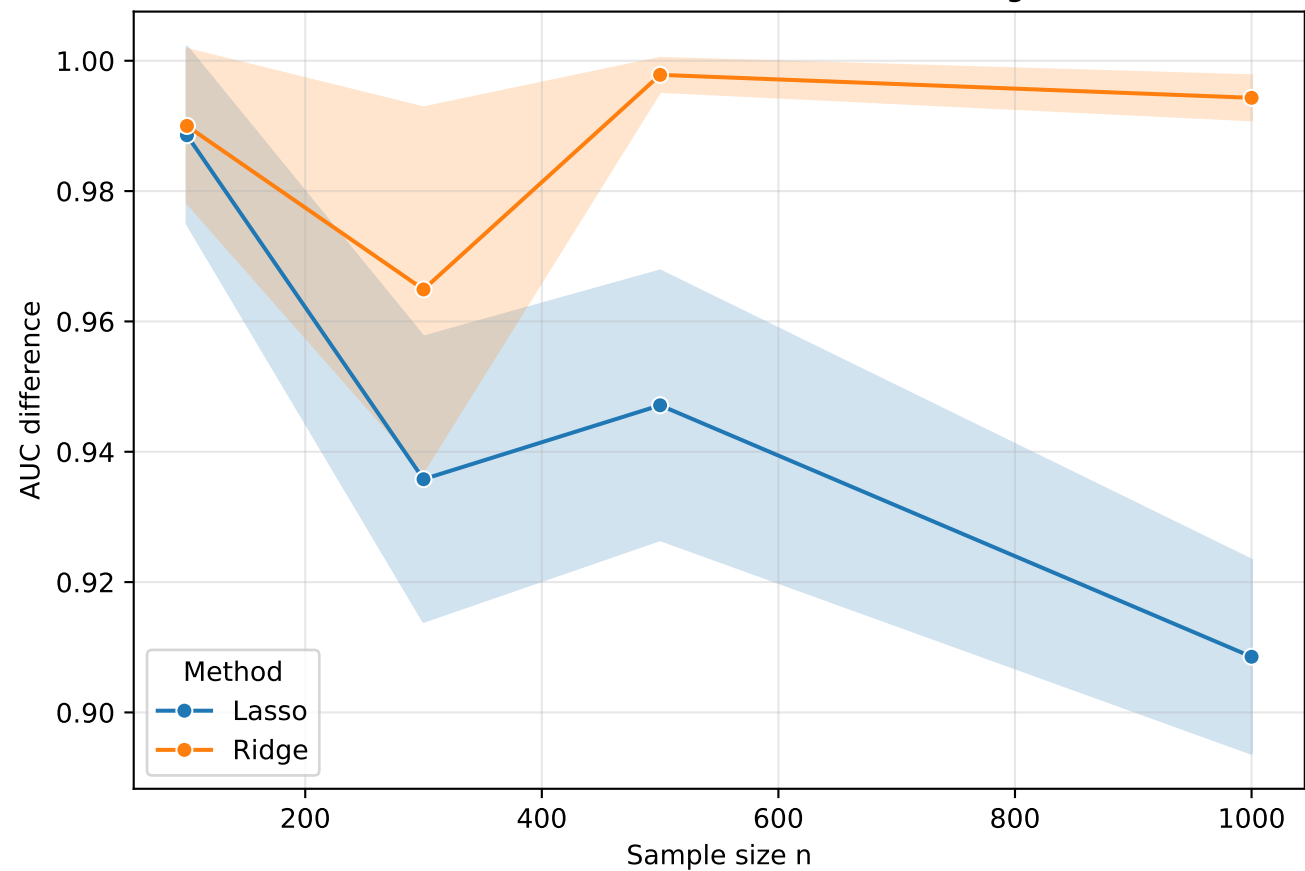
AUC difference vs. n for Lasso and Ridge
