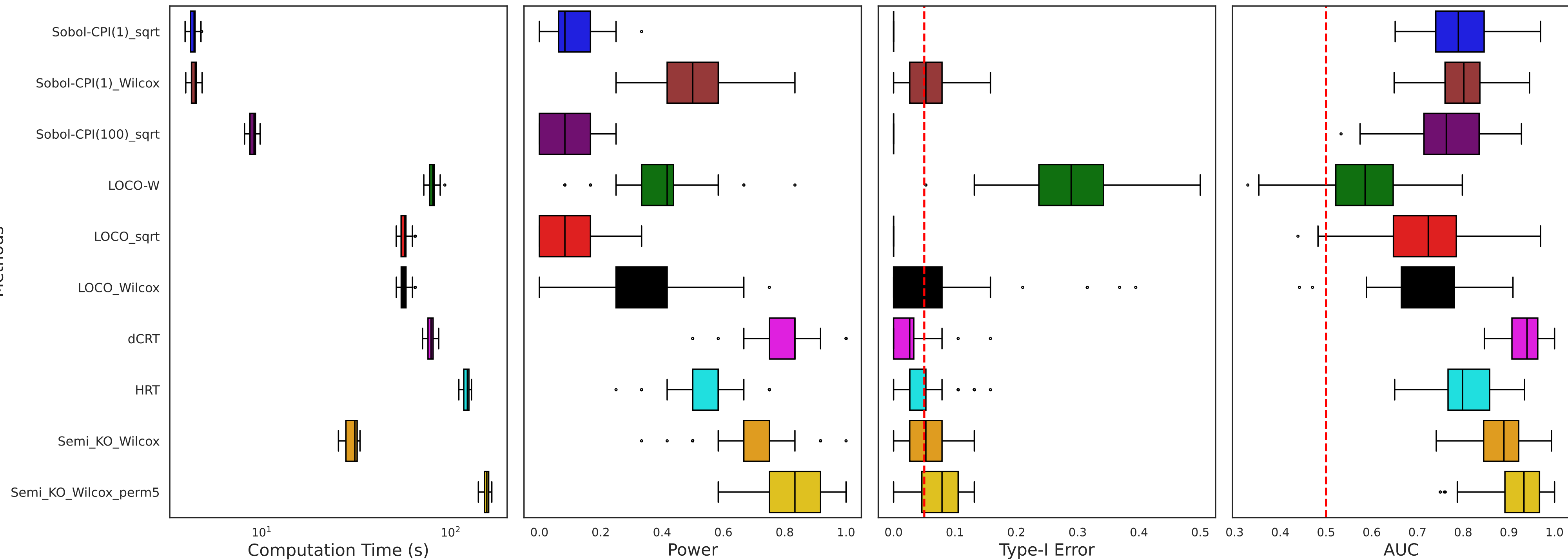
Inference Results ( R^2 HRT=0.655, R^2 Semi_KO=0.696)
