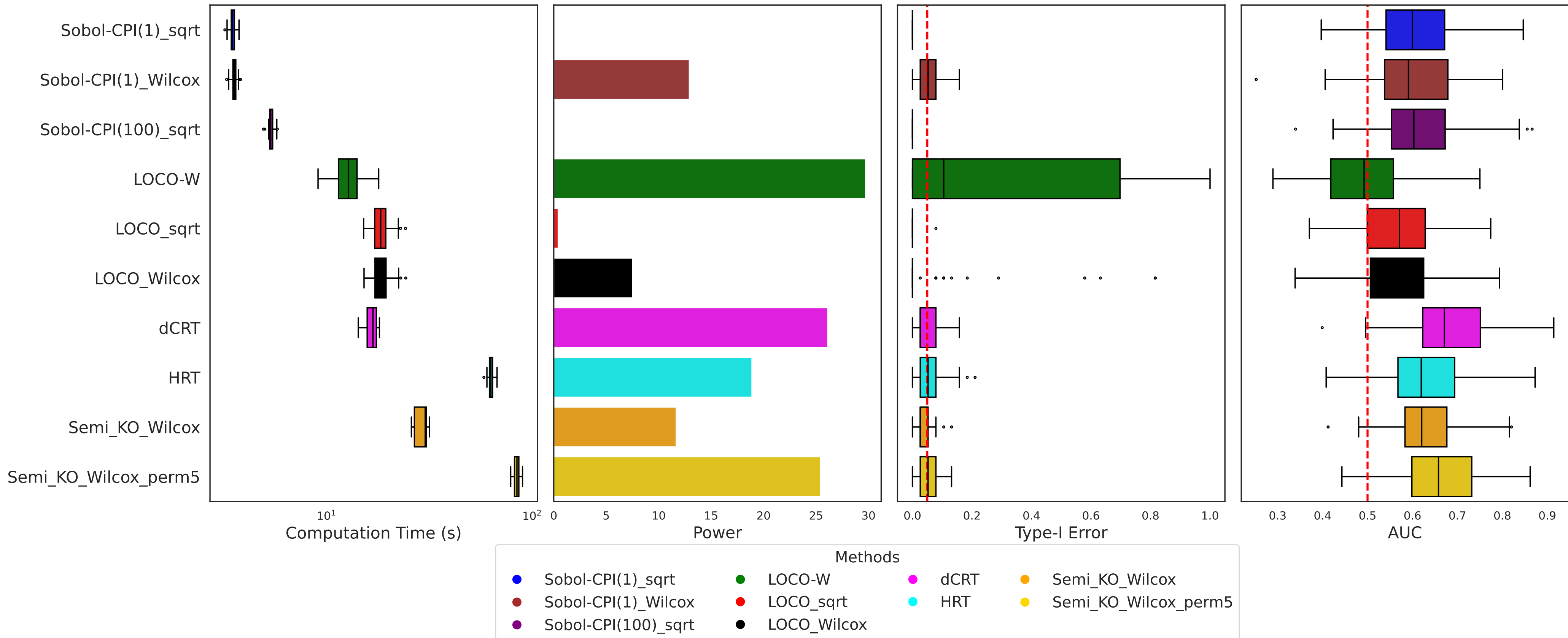
Inference Results (R2 HRT=-0.032, R2 Semi_KO=-0.001)
