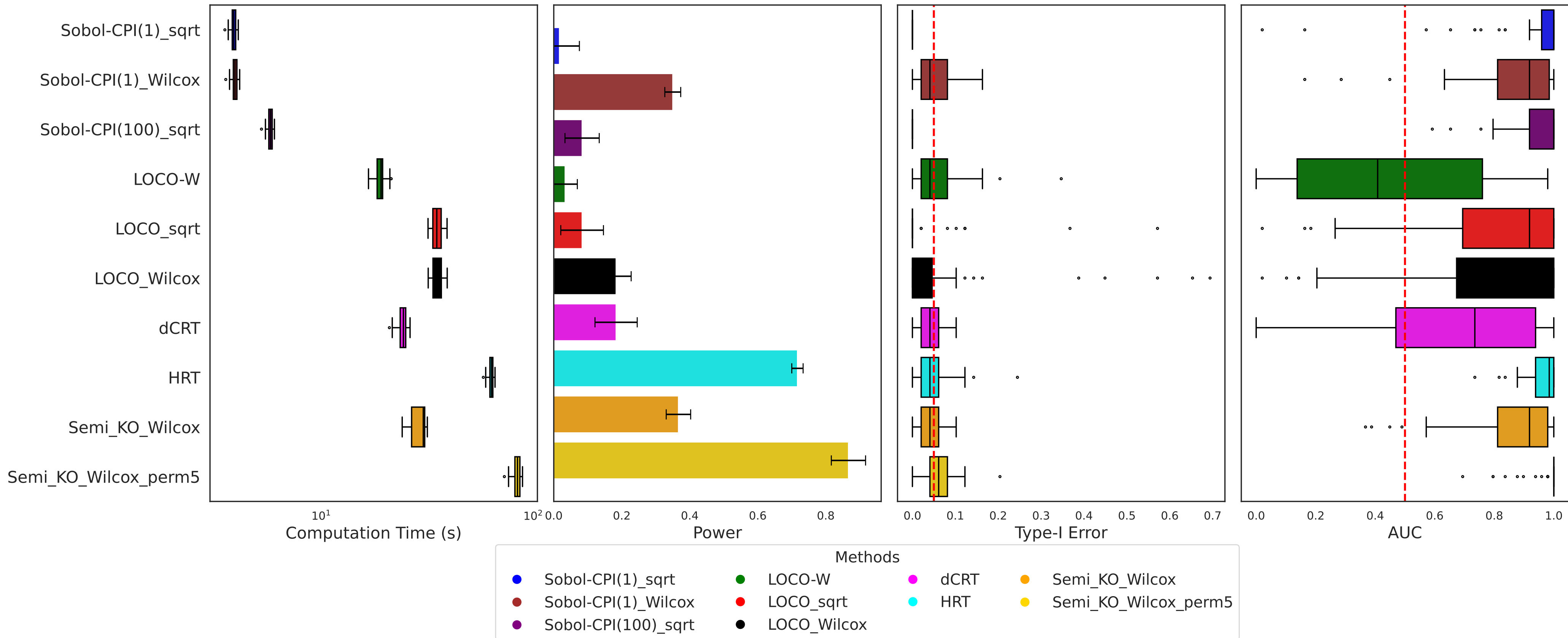
Inference Results ( R^2 HRT=-0.301, R^2 Semi_KO=-0.339)
