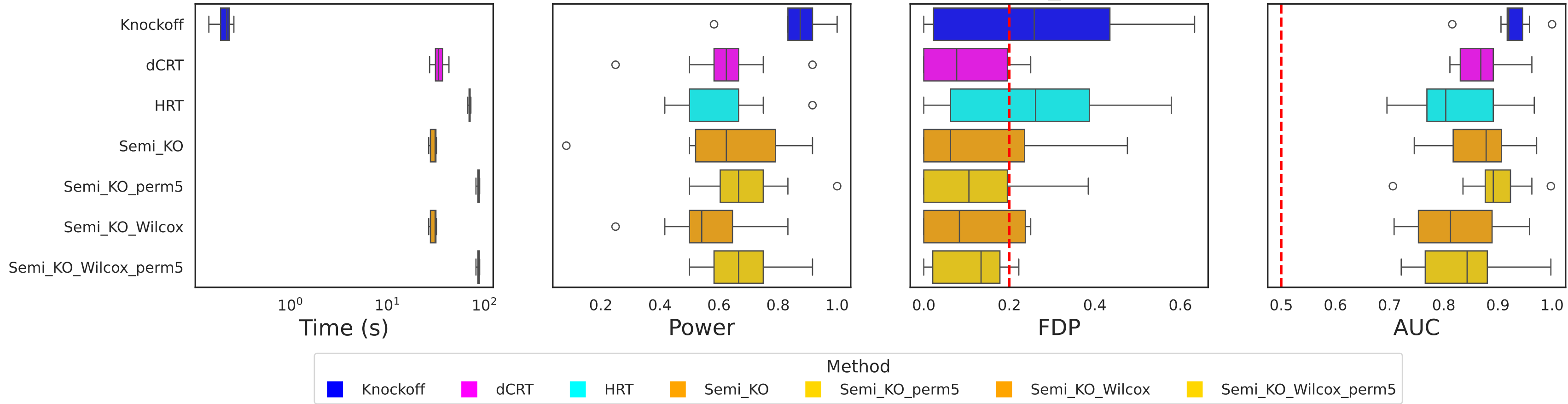
Inference Results (R2 HRT=0.832, R2 Semi_KO=0.854)
