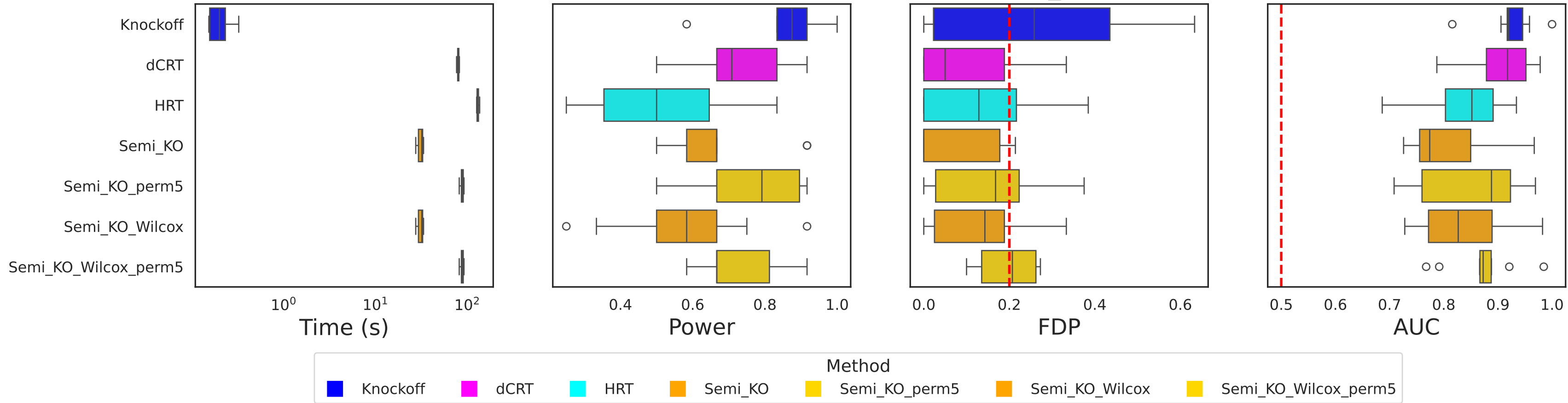
Inference Results (R2 HRT=0.740, R2 Semi_KO=0.787)
