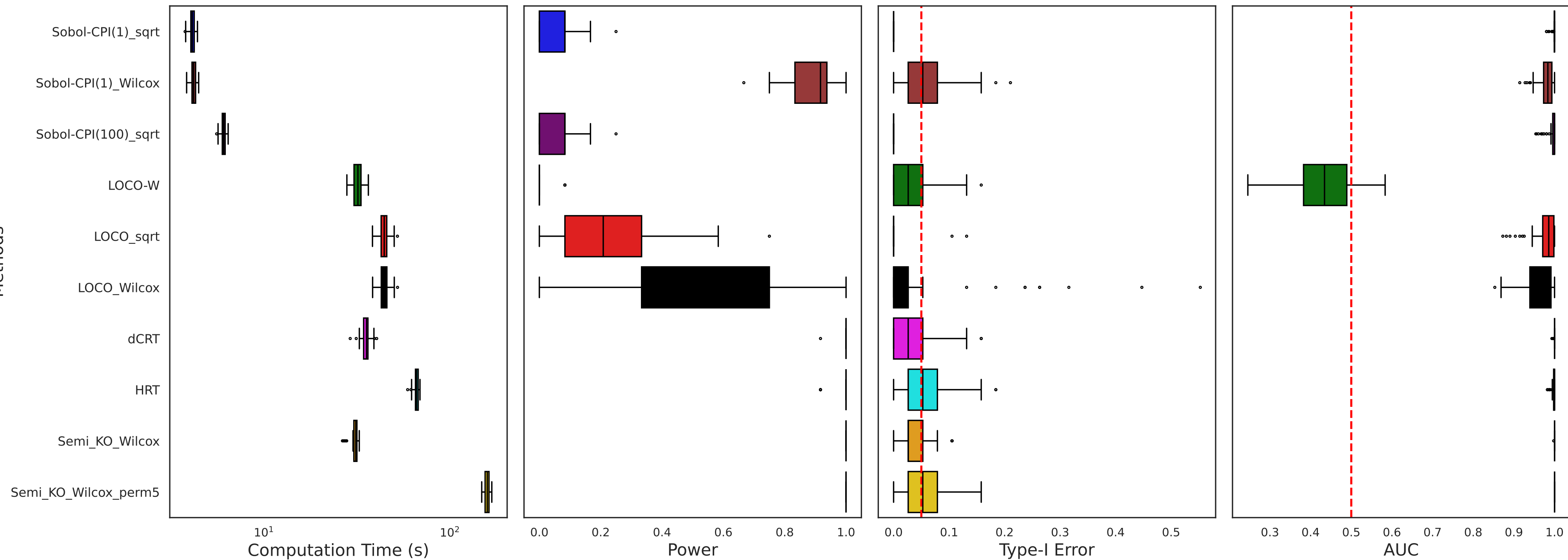
Inference Results ( R^2 HRT=0.893, R^2 Semi_KO=0.912)
