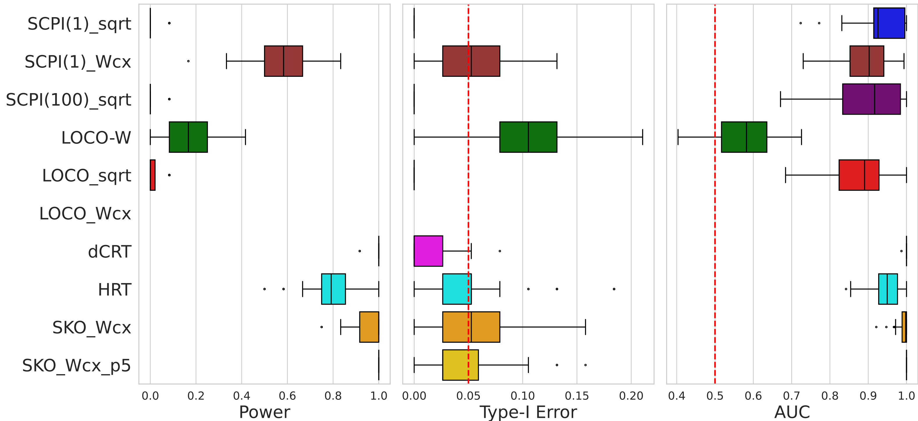
Inference Results (R2 HRT=0.799, R2 SKO=0.825)
