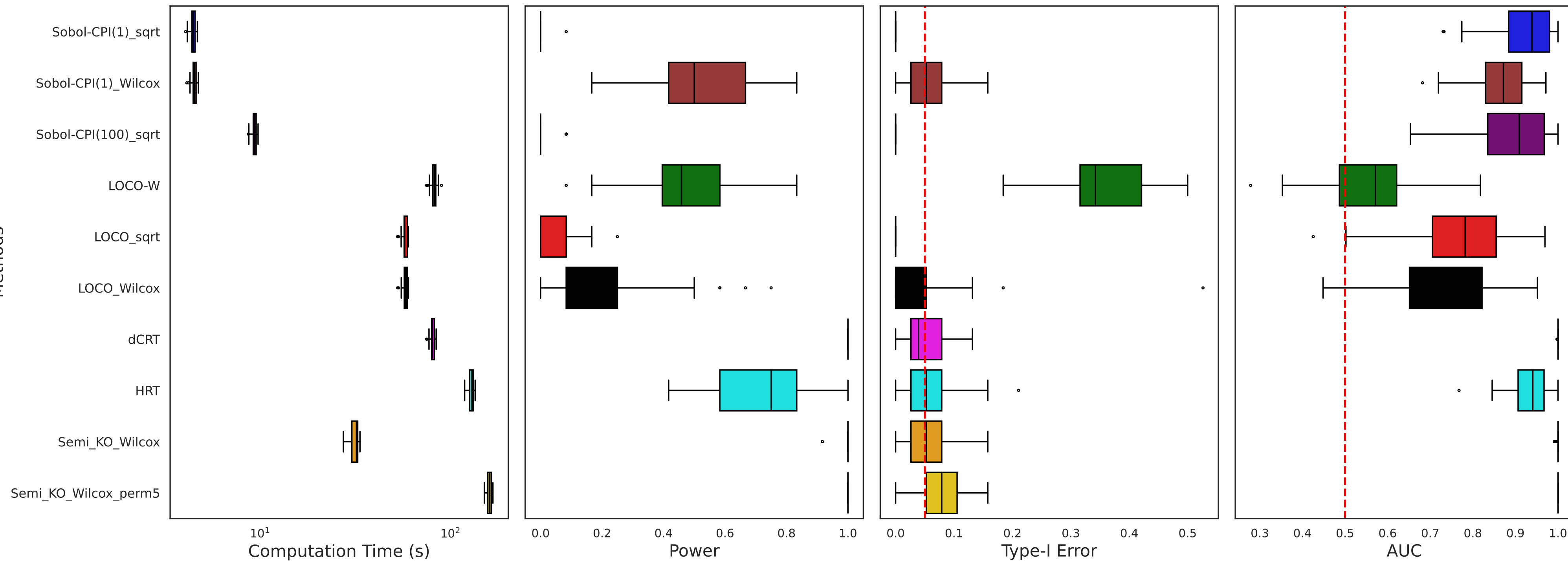
Inference Results ( R^2 HRT=0.683, R^2 Semi_KO=0.742)
