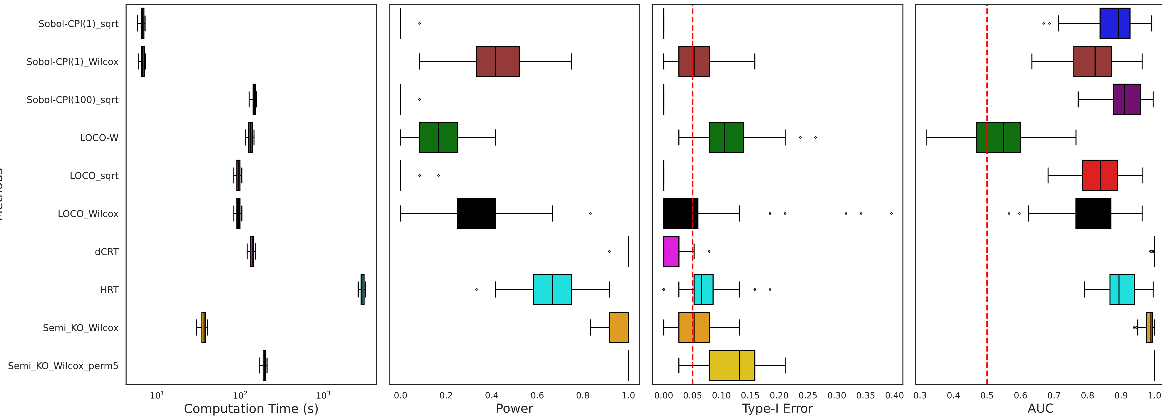
Inference Results ( R^2 HRT=0.541, R^2 Semi_KO=0.572)
