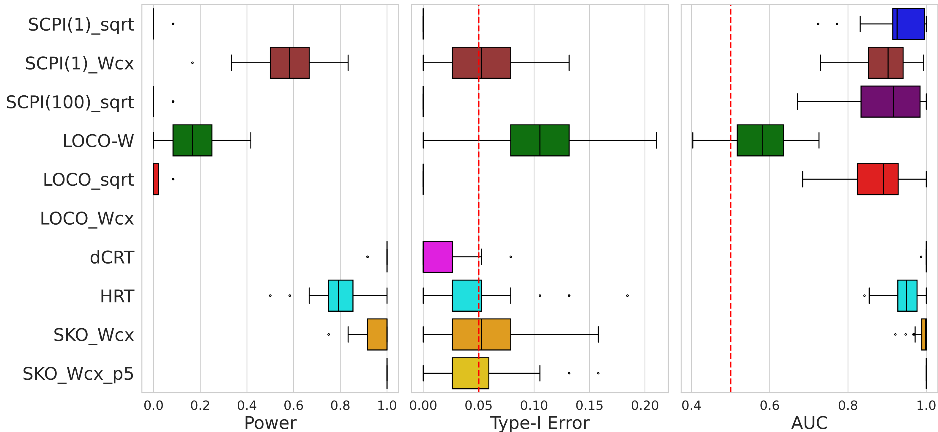
Inference Results (R2 HRT=0.799, R2 SKO=0.825)
