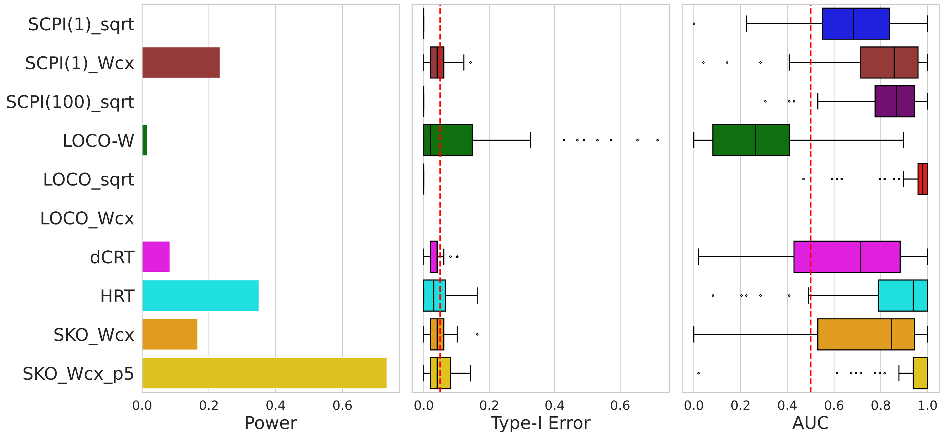
Inference Results (R2 HRT=0.567, R2 SKO=0.581)
