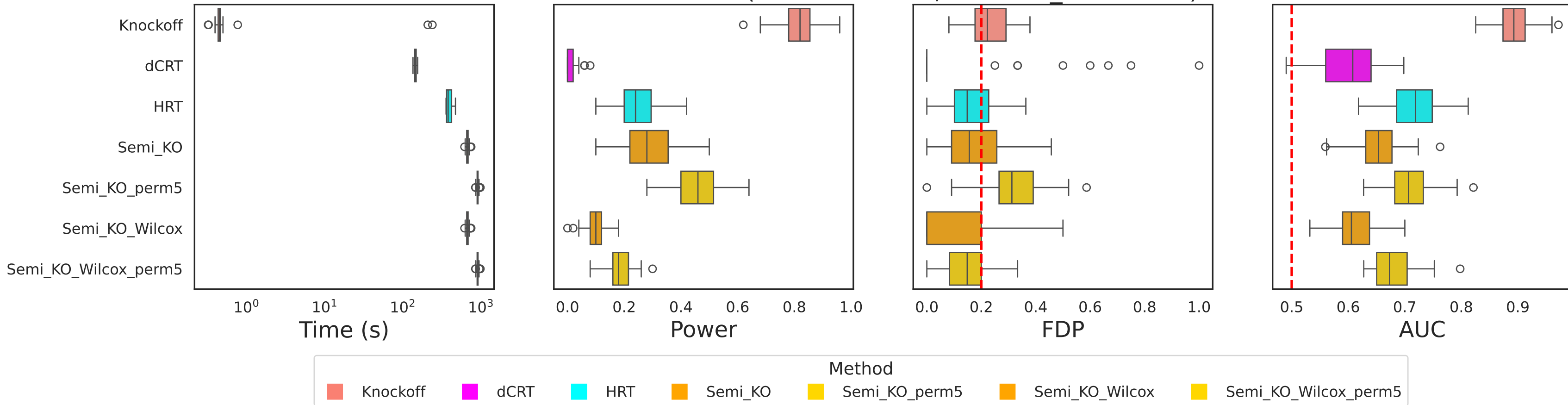
Inference Results ( R^2 HRT=0.597, R^2 Semi_KO=0.655)
