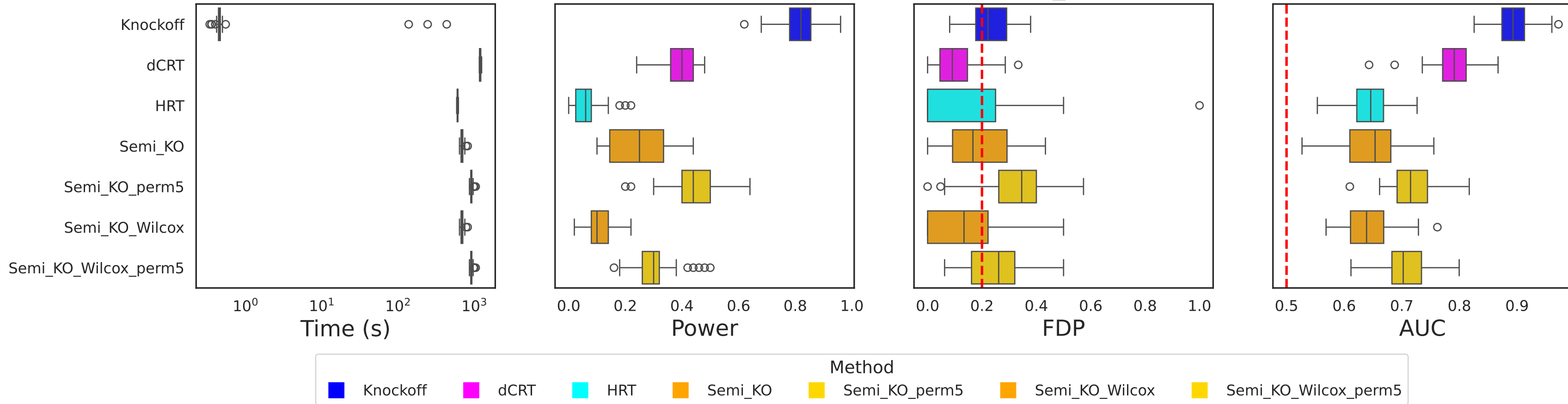
Inference Results (R2 HRT=0.431, R2 Semi_KO=0.513)
