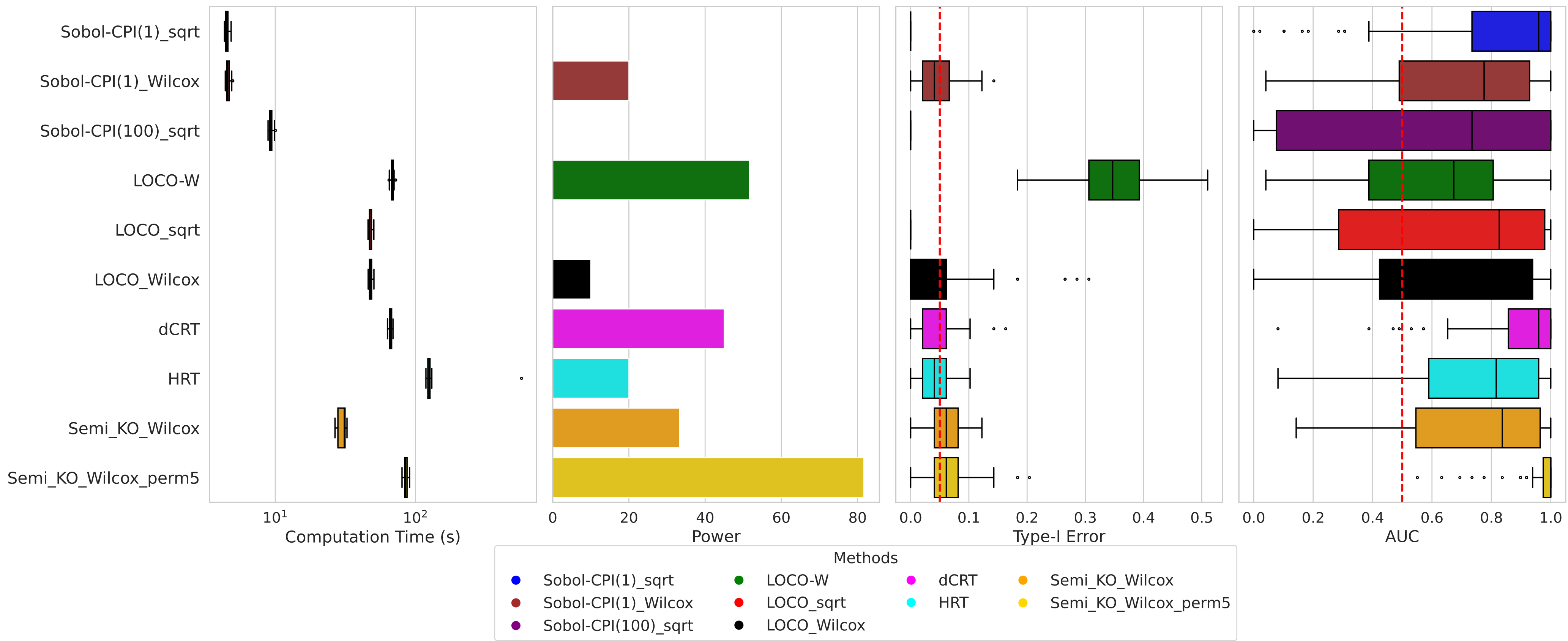
Inference Results (R2 HRT=0.735, R2 Semi_KO=0.744)
