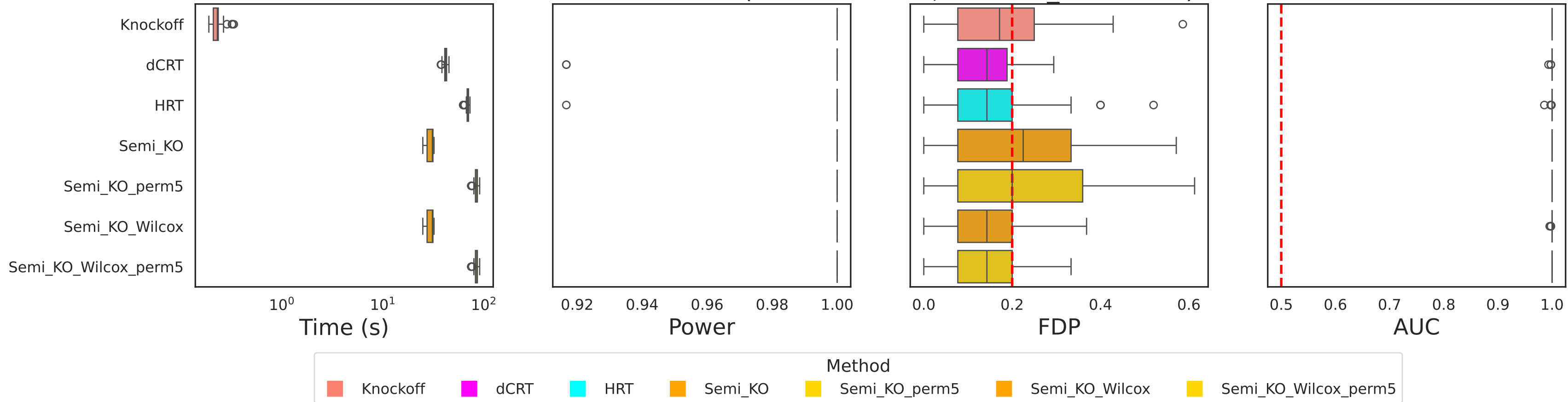
Inference Results ( R^2 HRT=0.964, R^2 Semi_KO=0.965)
