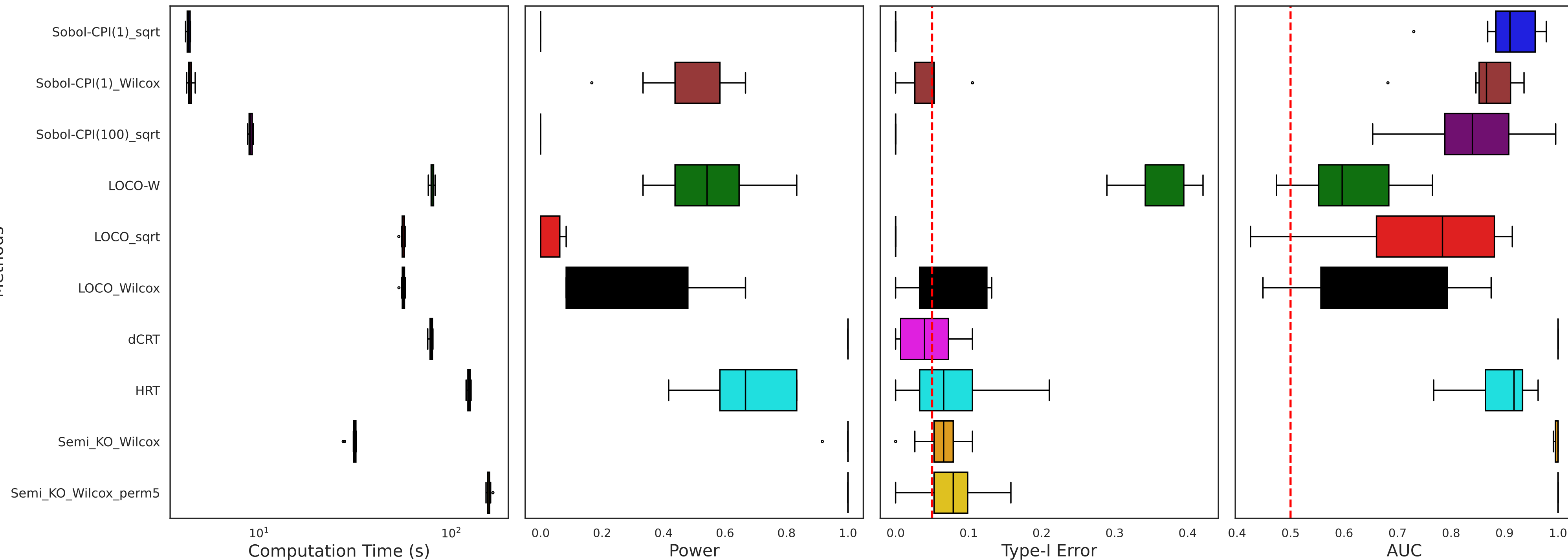
Inference Results (R2 HRT=0.686, R2 Semi_KO=0.740)
