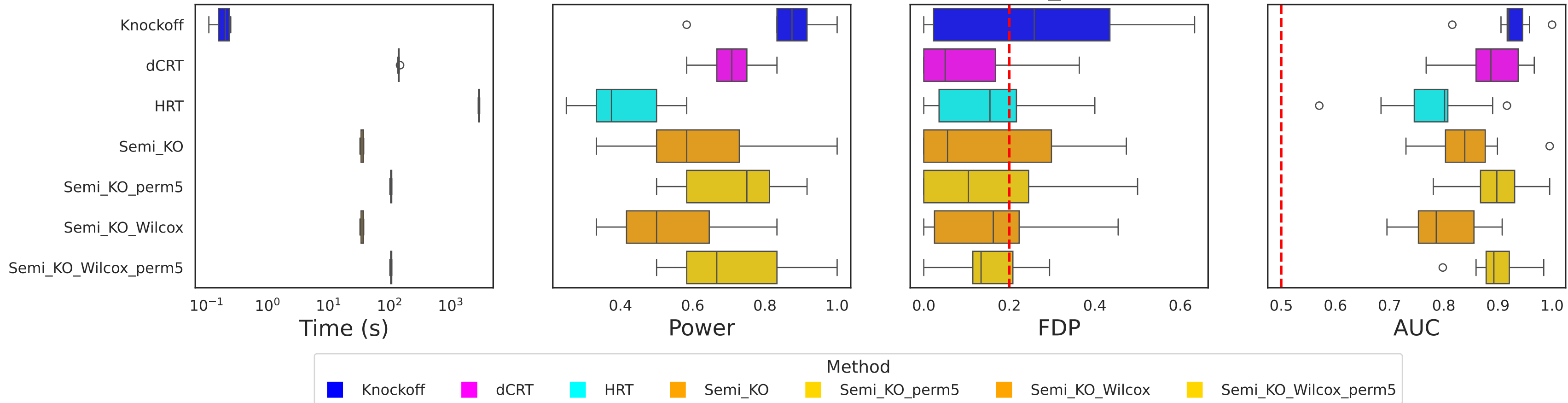
Inference Results (R2 HRT=0.661, R2 Semi_KO=0.706)
