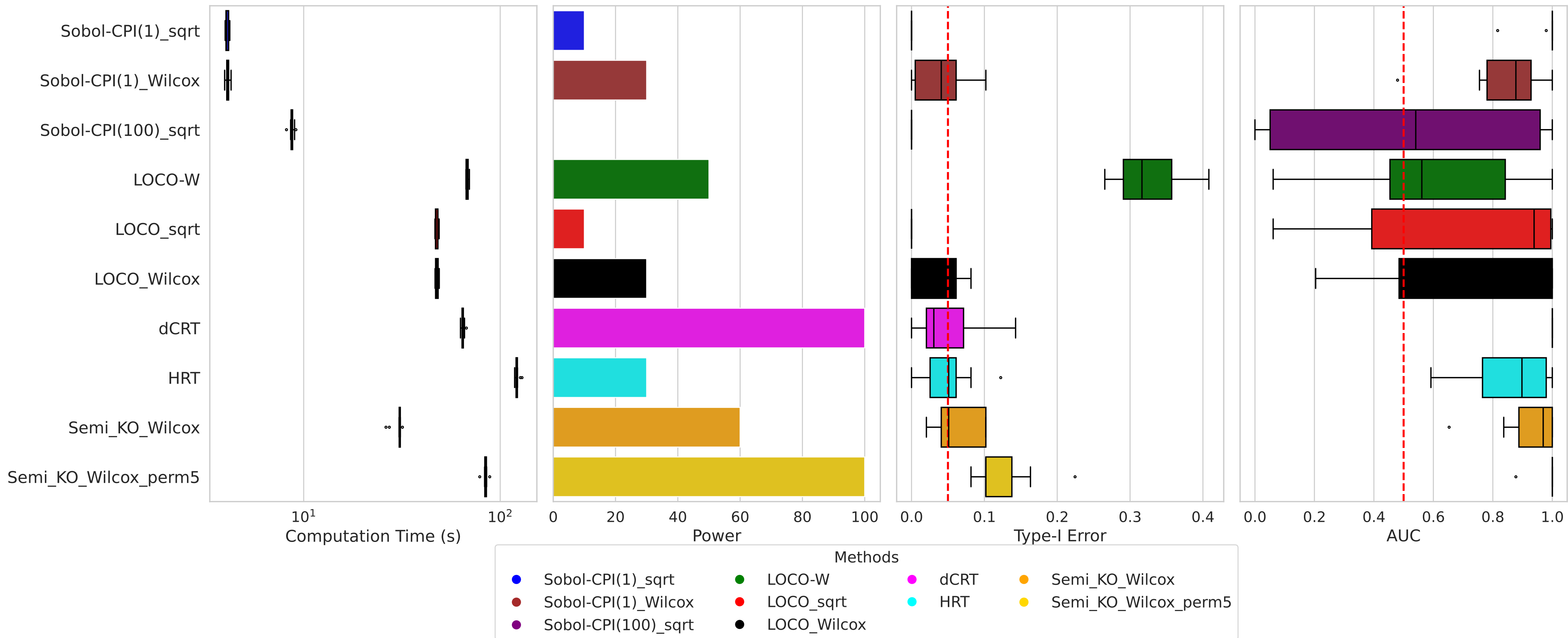
Inference Results (R2 HRT=-0.015, R2 Semi_KO=-0.011)
