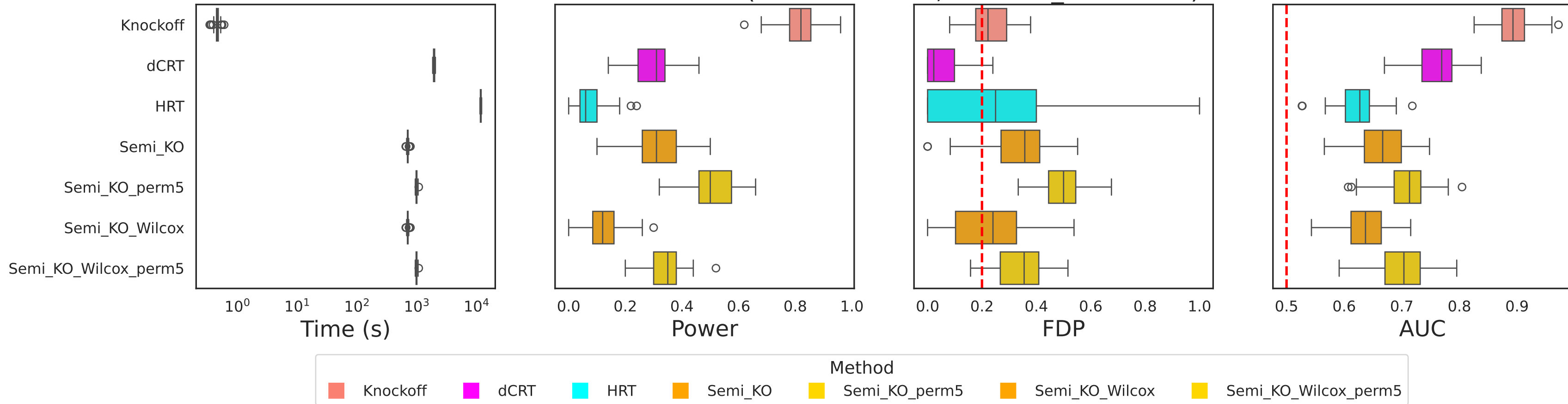
Inference Results ( R^2 HRT=0.314, R^2 Semi_KO=0.350)
