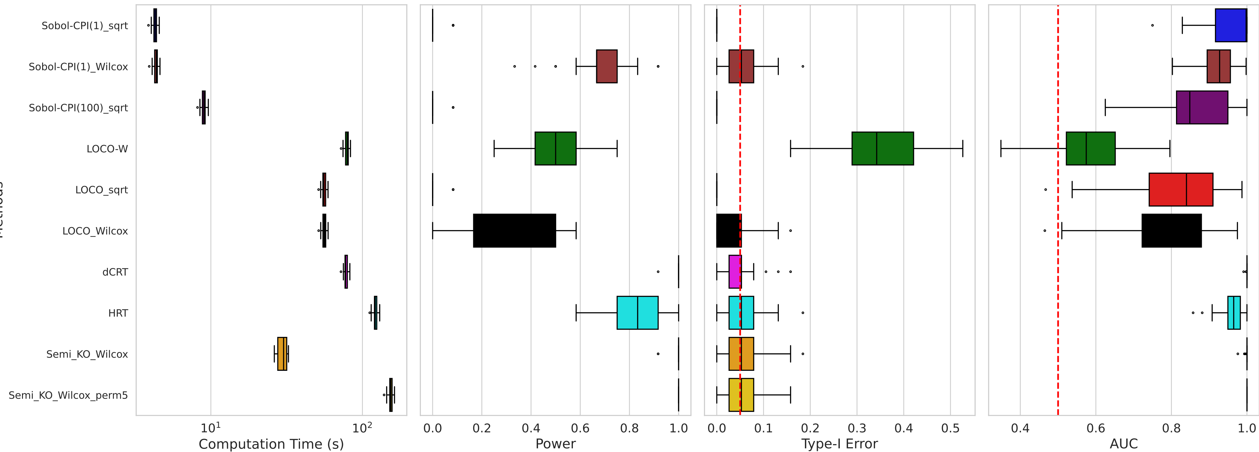
Inference Results (R2 HRT=0.887, R2 Semi_KO=0.910)
