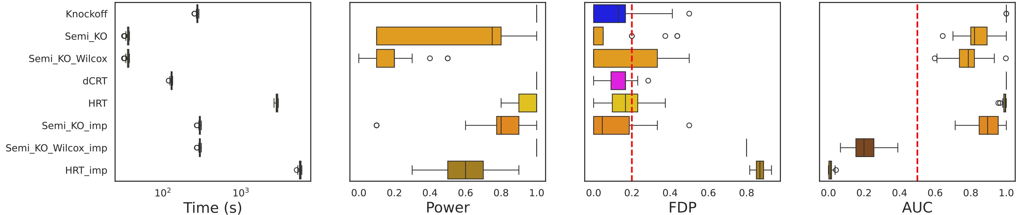
Method
