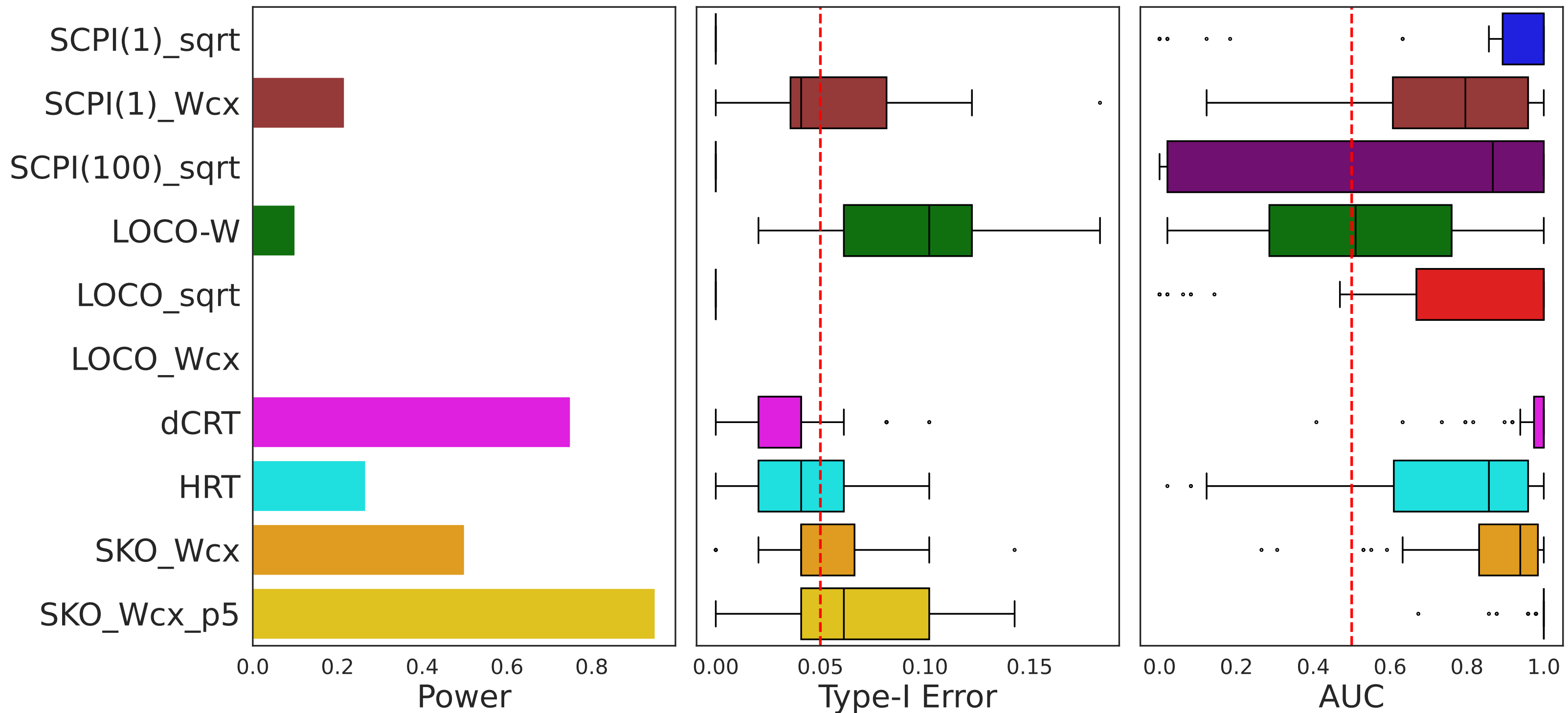
Inference Results (R2 HRT=0.760, R2 SKO=0.768)
