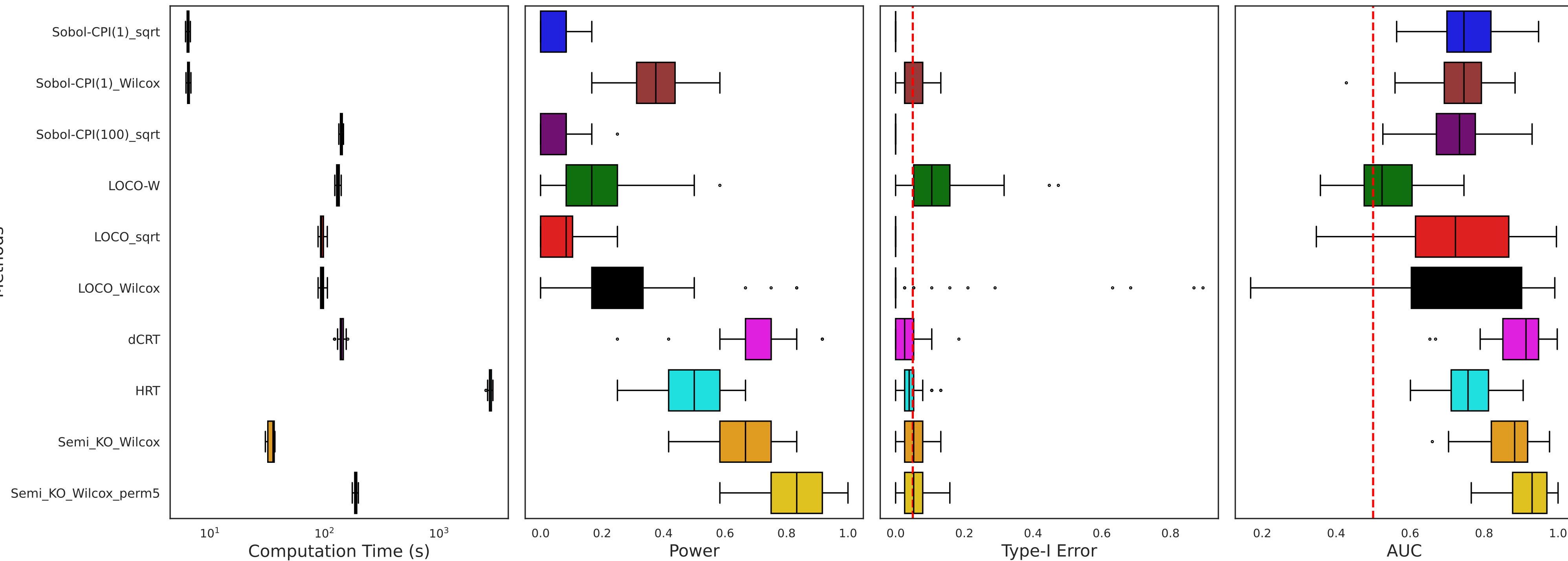
Inference Results ( R^2 HRT=0.556, R^2 Semi_KO=0.599)
