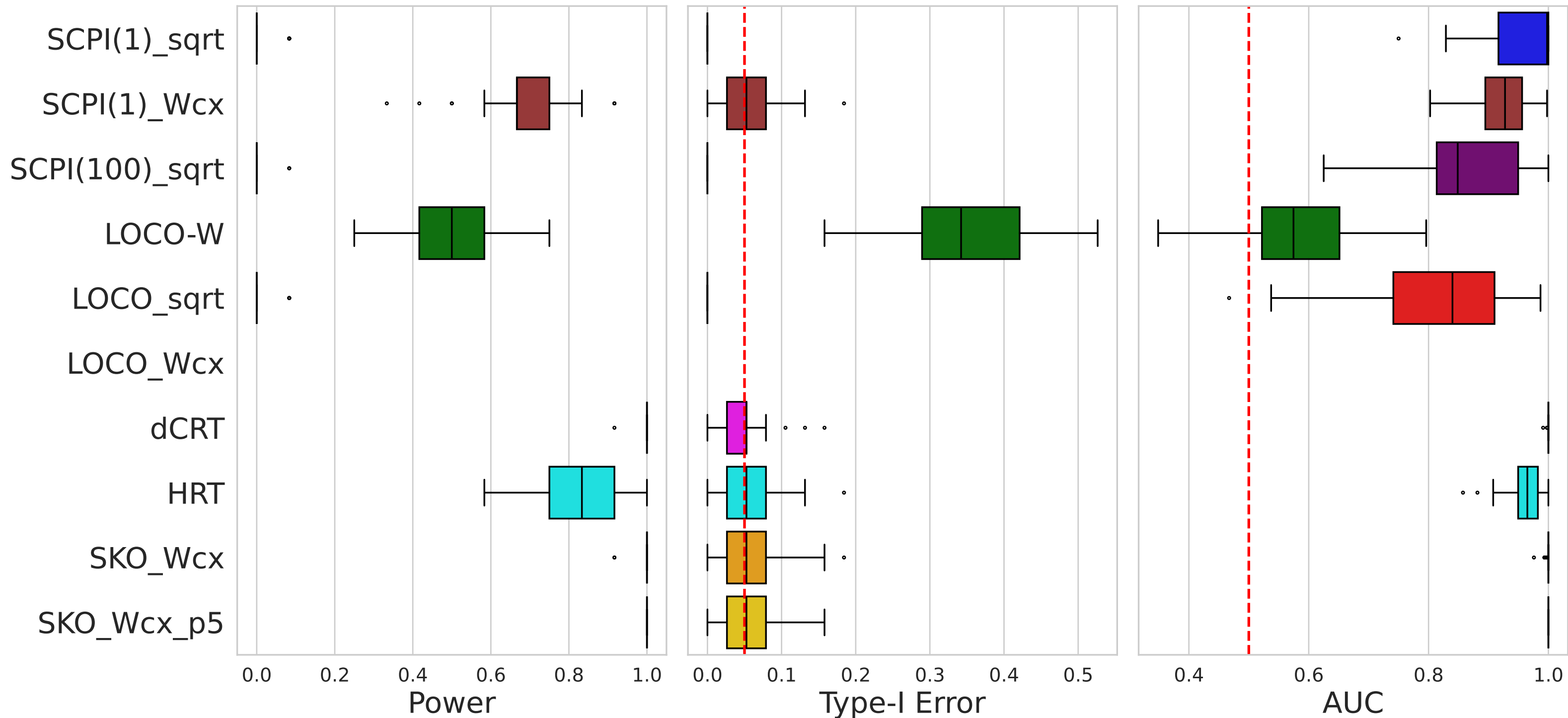
Inference Results (R2 HRT=0.887, R2 SKO=0.910)
