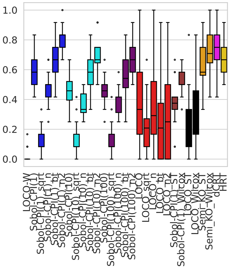
Power
