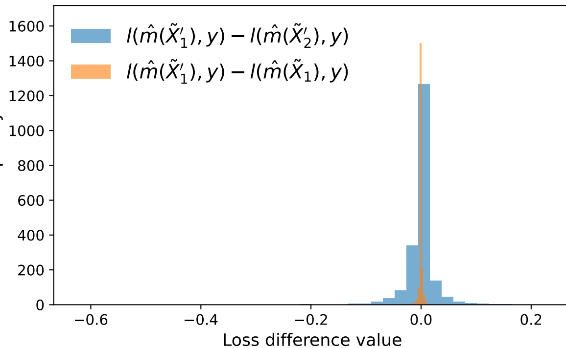
Random Forest
