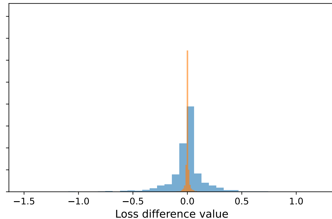
Neural Network
