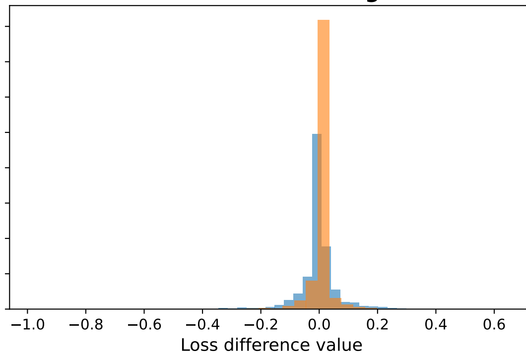
Gradient Boosting
