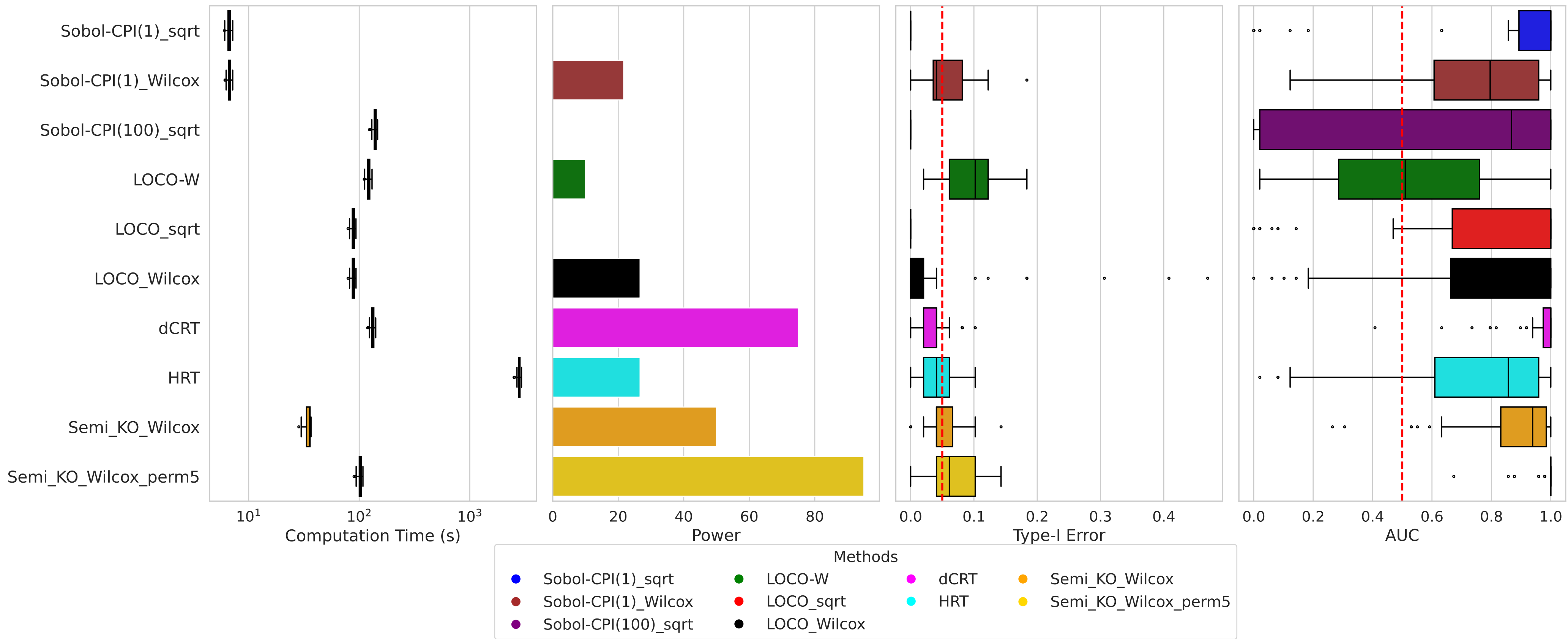
Inference Results (R2 HRT=0.760, R2 Semi_KO=0.768)
