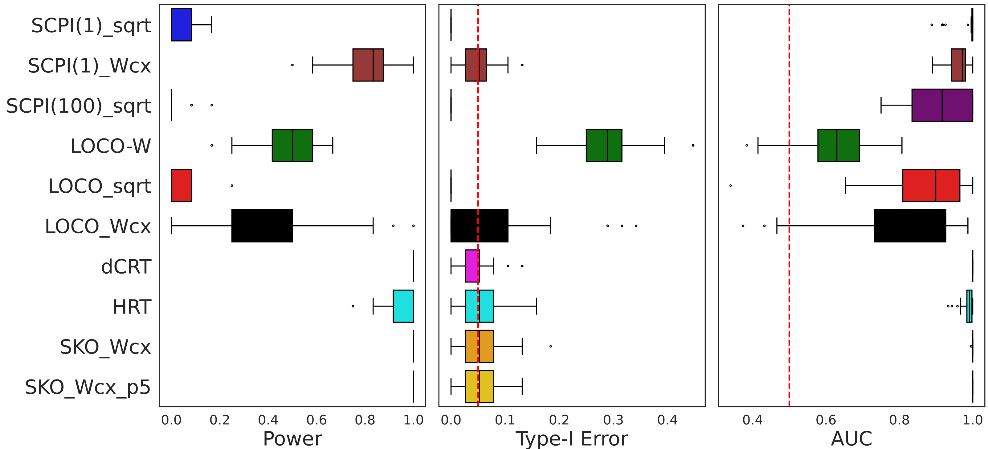
Inference Results ( R^2 HRT=0.908, R^2 SKO=0.925)
