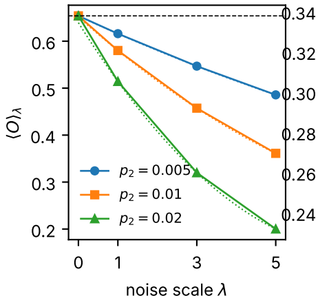
TFIM, 5 Trotter steps
