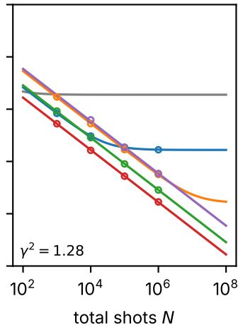
GHZ n=6 , p_2=0.01
