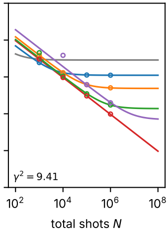
TFIM d=10 , p_2=0.01
