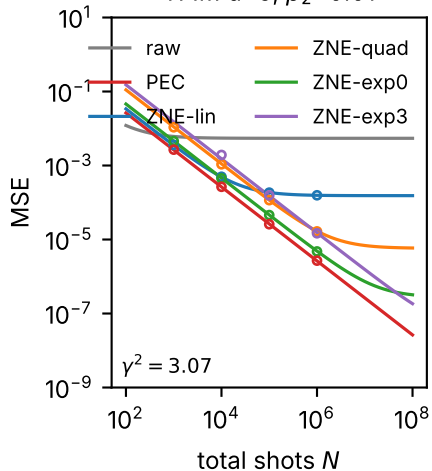
TFIM d=5 , p_2=0.01
