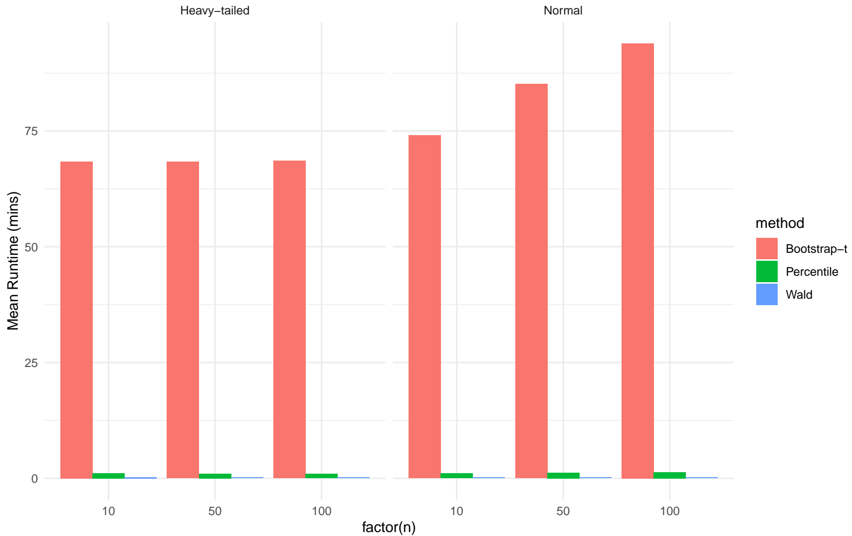
Average Runtime per Scenario (Averaged over Beta values)
