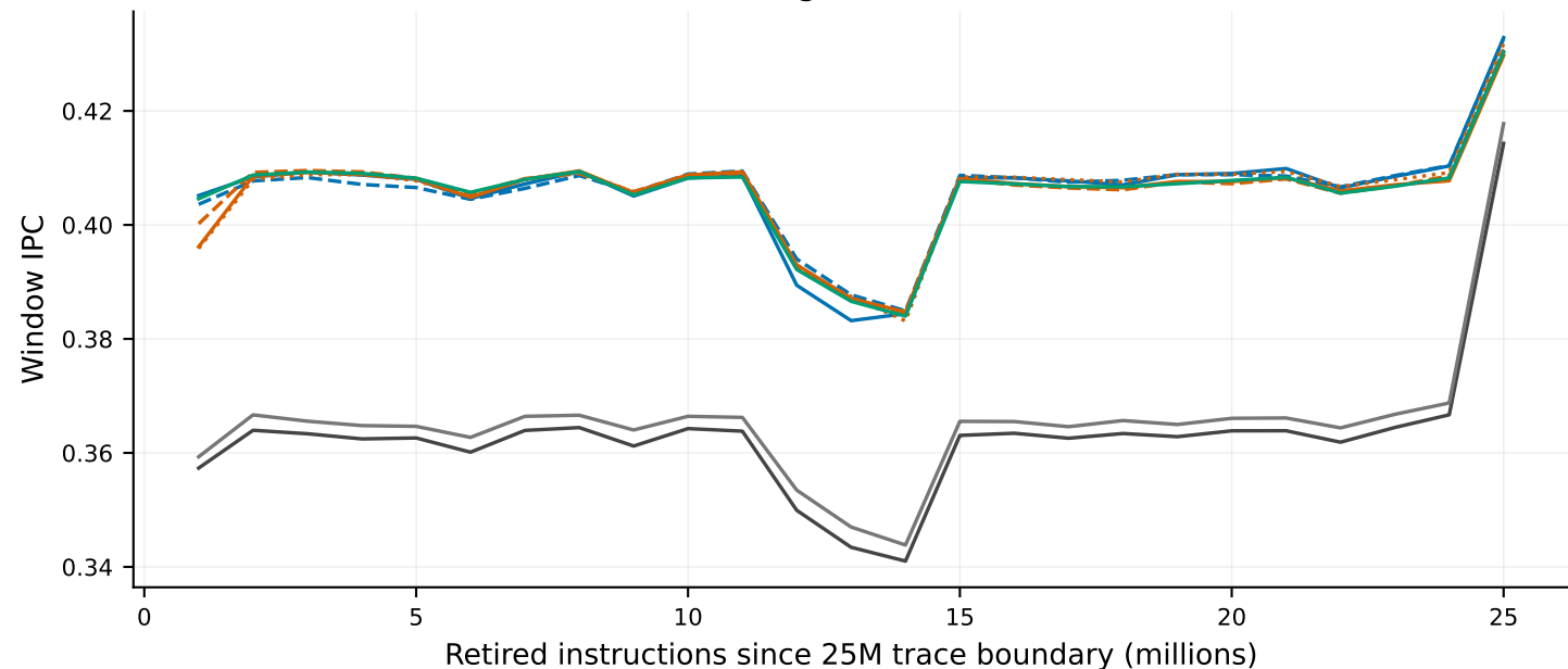
h8: online learning and frozen references
