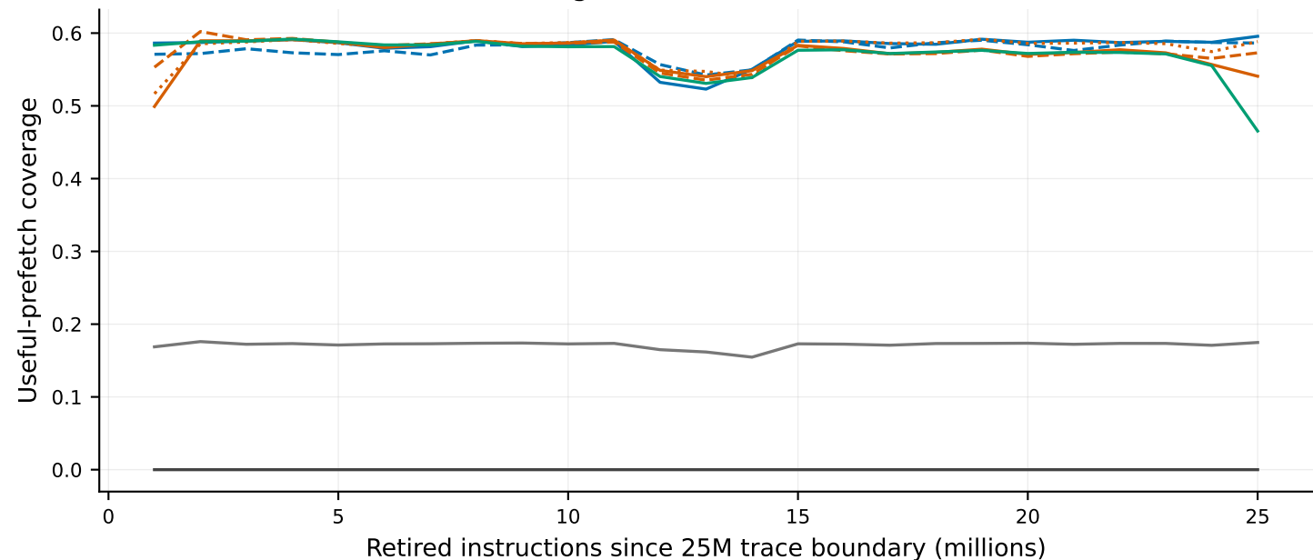
h8: coverage in 1M instruction windows
