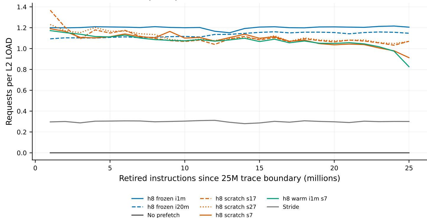
h8: request pressure in 1M instruction windows
