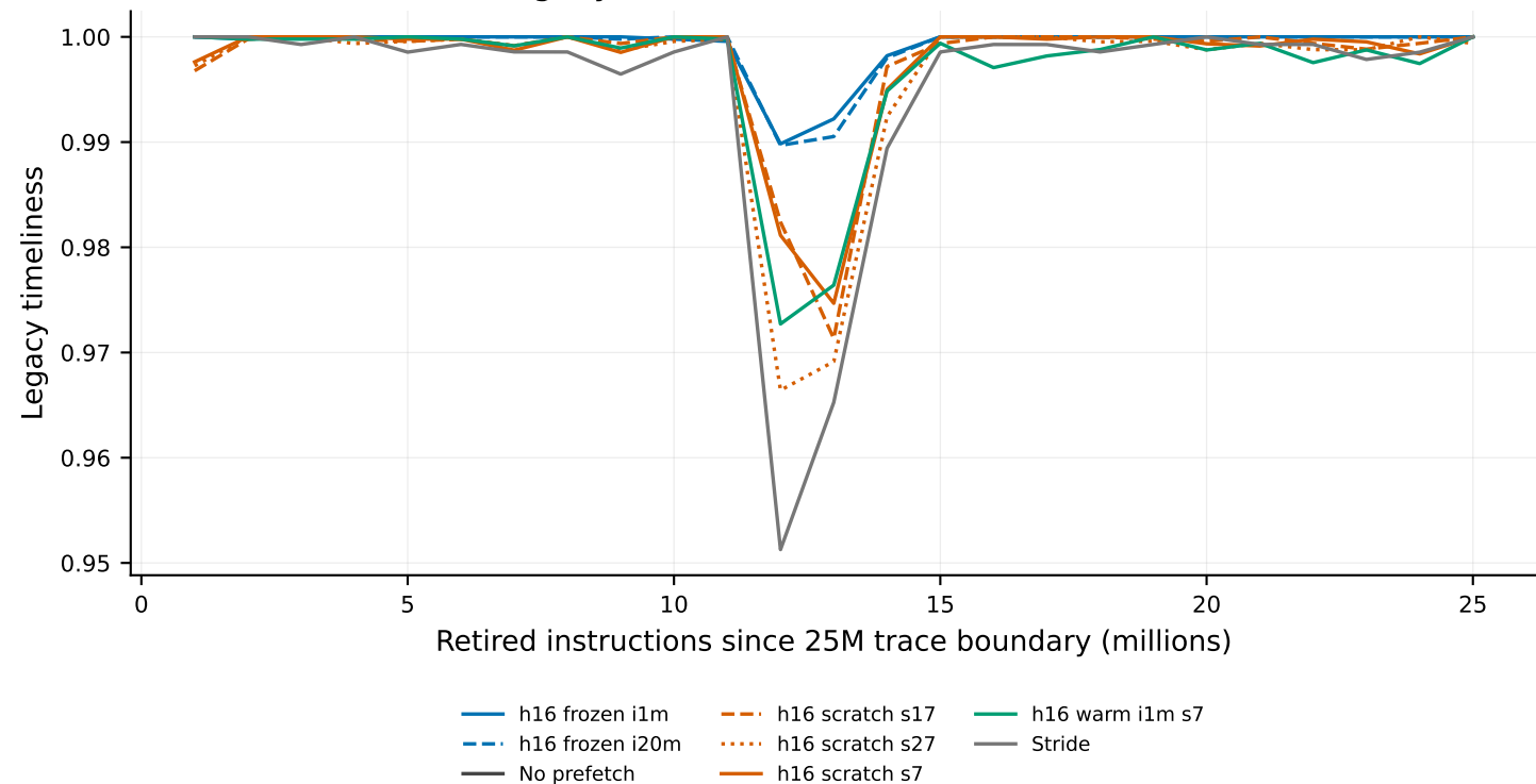
h16: legacy timeliness in 1M instruction windows
