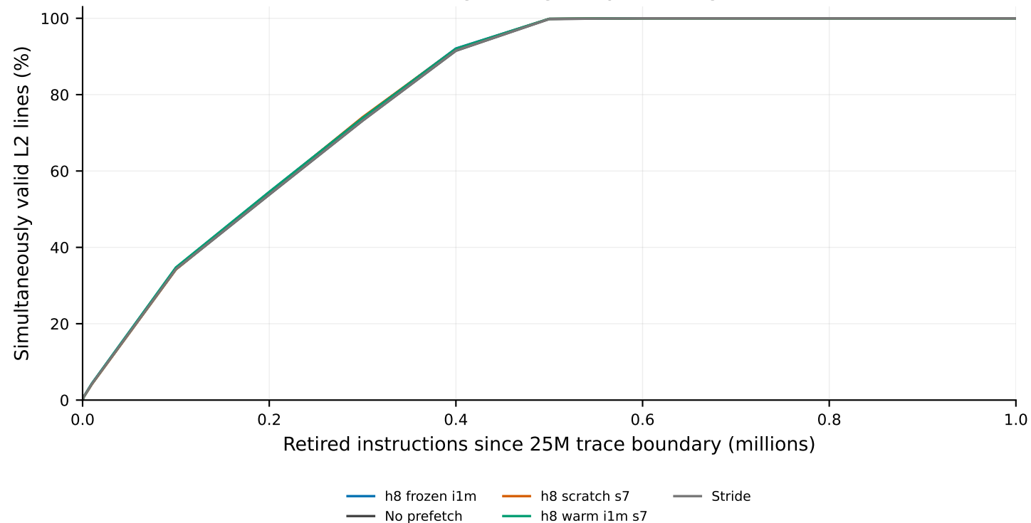
L2 filling during early learning
