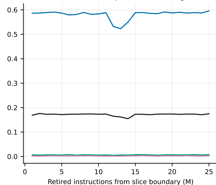
Window useful-prefetch coverage
