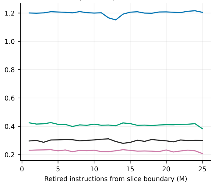
Window requested prefetches / L2 LOAD
