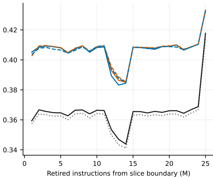
Window useful-prefetch coverage
