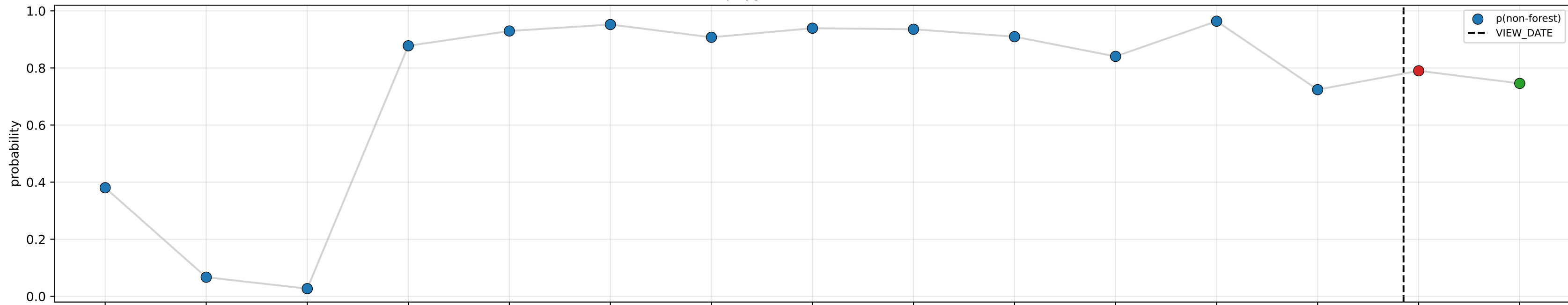
fid 389 - Degradation - joint_binary / log_reg 7 polygon tokens over 1x1 tiles
