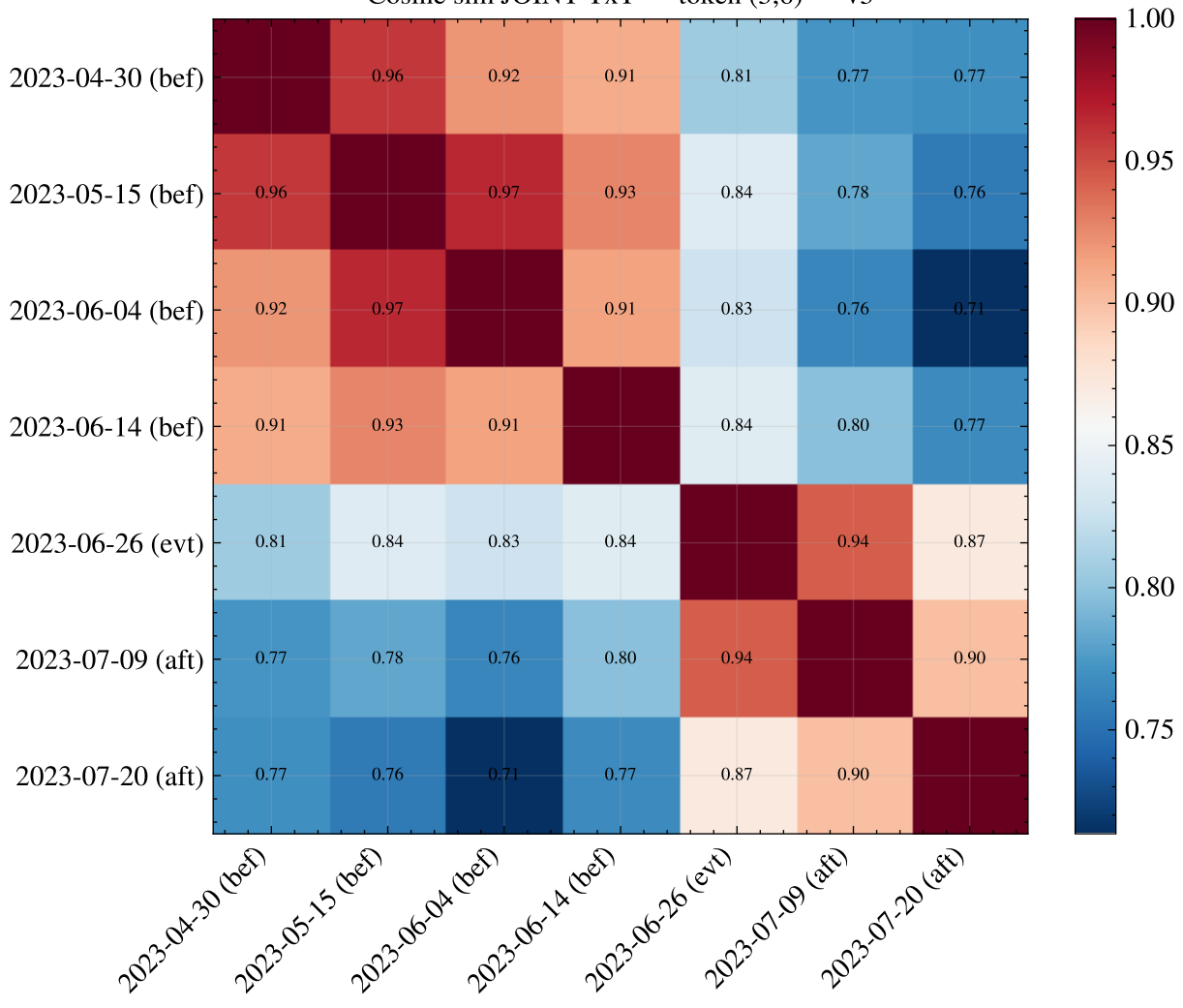
Cosine sim JOINT TxT — token (3,6) — v3
