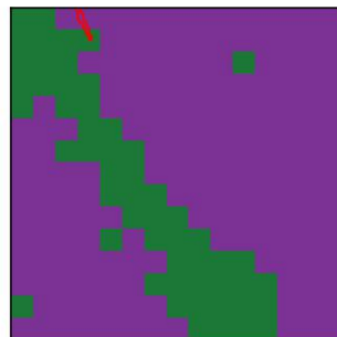
LogisticRegression
