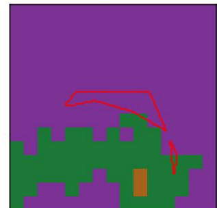
RandomForest
