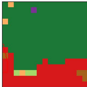
LogisticRegression
