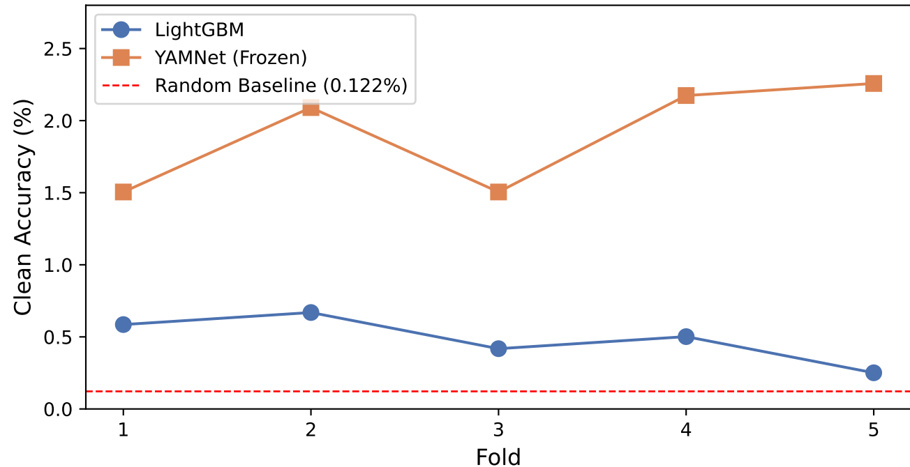
5-Fold Cross-Validation Clean Accuracy
