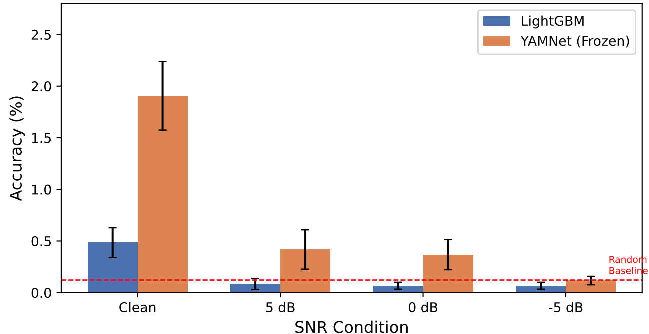
Noise Robustness: LightGBM vs YAMNet (Frozen)
