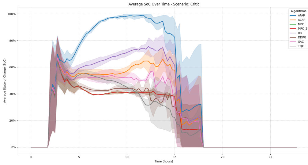
Figure 3.11: Average State of Charge (SoC) of all connected EVs over time.
