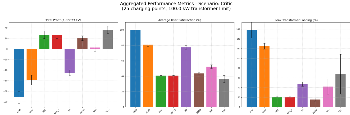
Figure 3.8: Overall performance summary comparing all algorithms across key metrics.
