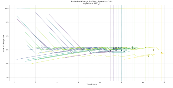
(a) Individual ev profiles for Adaptive MPC: it slightly charges at times, but occasionally exhibits a negative ramp due to discharging.
