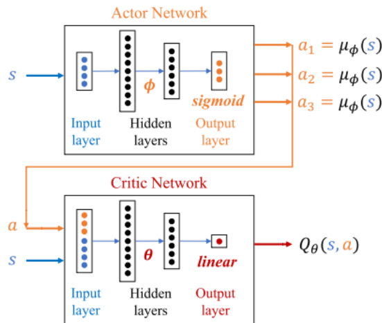
Figure 3.4: DDPG architecture.
