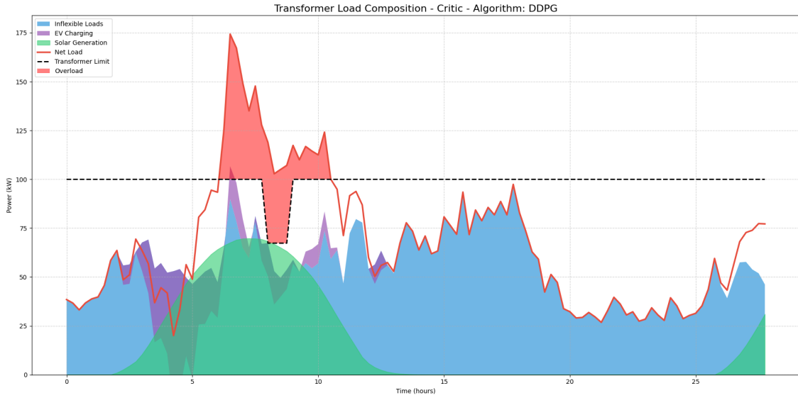
Figure 3.15: Overload composition for DDPG algorithm.
