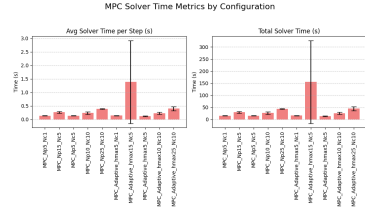
(c) Solver time.
