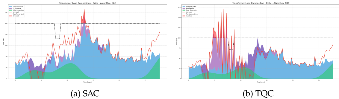
Figure 3.13: Grid load for SAC and TQC RL algorithms. The SAC agents learn to respect the grid constraints better than TQC.
