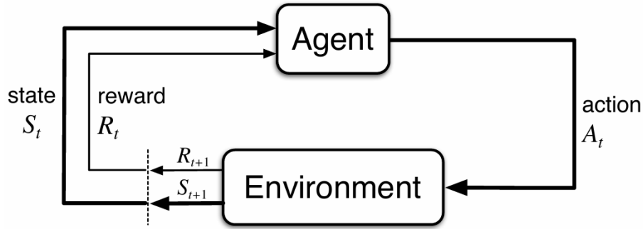
Figure 2.6: The agent-environment interaction loop in reinforcement learning [45].
