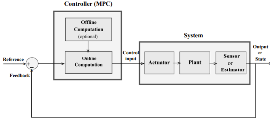
Figure 2.11: MPC: Block diagram
