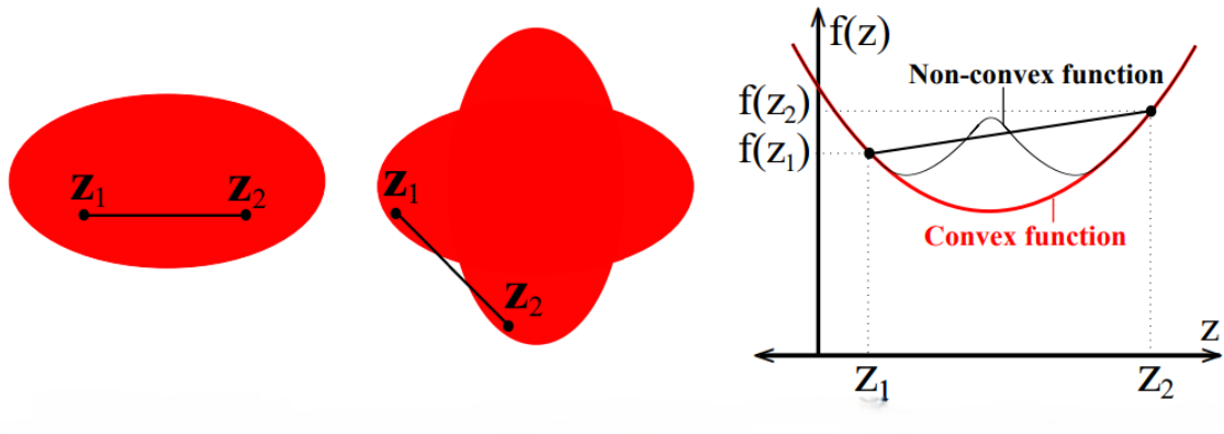
Figure 2.13: On the left, a convex set; in the middle, a non-convex set; on the right, a convex function.
