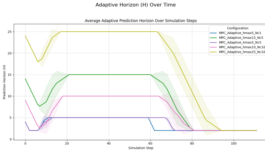
Figure 3.18: Adaptive horizon
