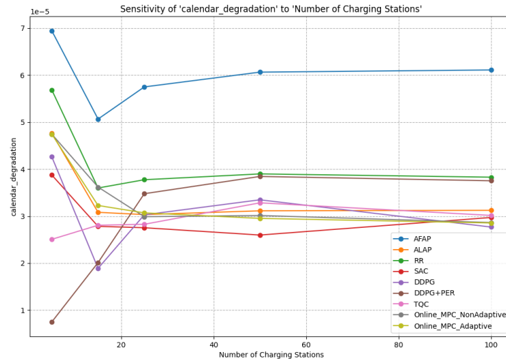
Figure 4.7: Sensitivity of Calendar Degradation to the Number of Charging Stations.
