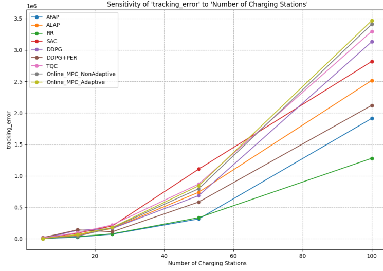
Figure 4.22: Sensitivity of Tracking Error to the Number of Charging Stations.
