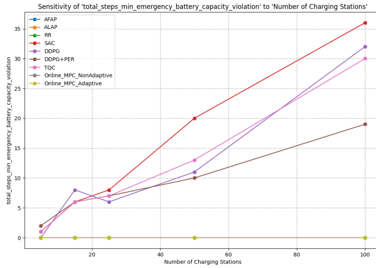
Figure 4.21: Sensitivity of Total Steps Min Emergency Battery Capacity Violation to the Number of Charging Stations.
