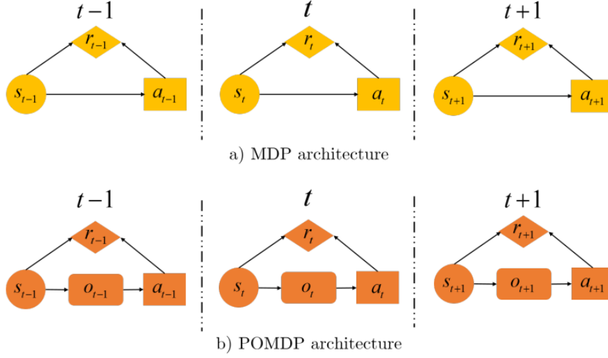
Figure 2.8: Differences between POMDP and MDP [38].
