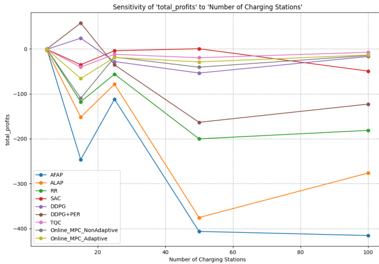
Figure 4.19: Sensitivity of Total Profits to the Number of Charging Stations.
