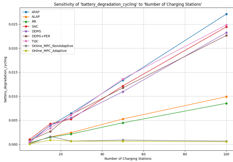
Figure 4.5: Sensitivity of Battery Degradation Cycling to the Number of Charging Stations.
