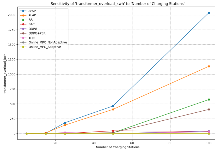
Figure 4.23: Sensitivity of Transformer Overload Kwh to the Number of Charging Stations.
