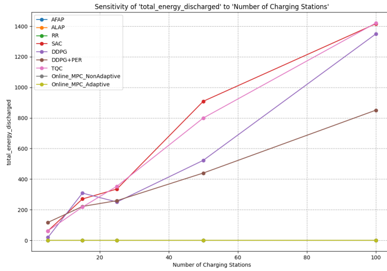
Figure 4.18: Sensitivity of Total Energy Discharged to the Number of Charging Stations.
