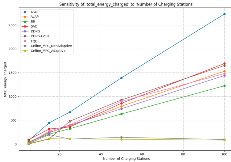
Figure 4.17: Sensitivity of Total Energy Charged to the Number of Charging Stations.
