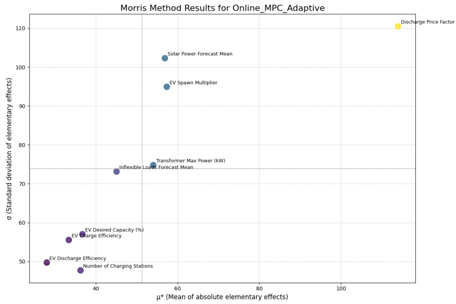
Figure 4.28: Morris method sensitivity plot for the Online MPC Adaptive algorithm.
