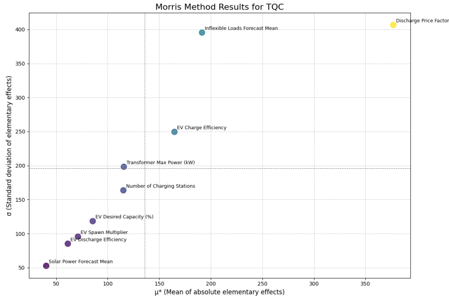
Figure 4.32: Morris method sensitivity plot for the TQC algorithm.
