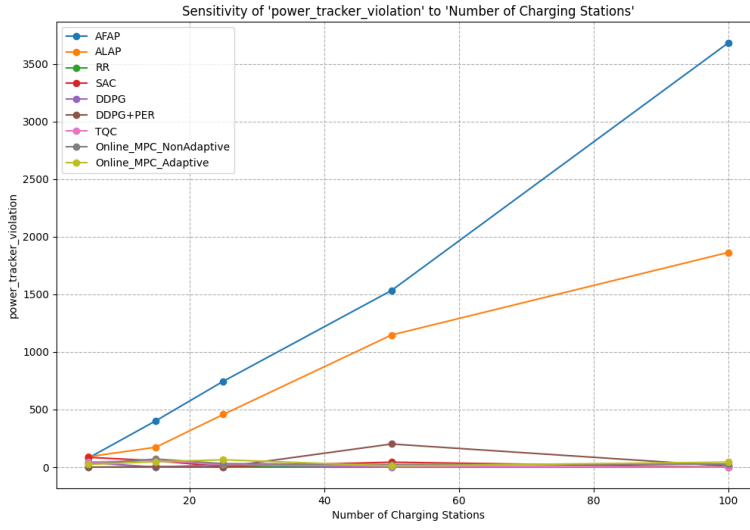
Figure 4.14: Sensitivity of Power Tracker Violation to the Number of Charging Stations.
