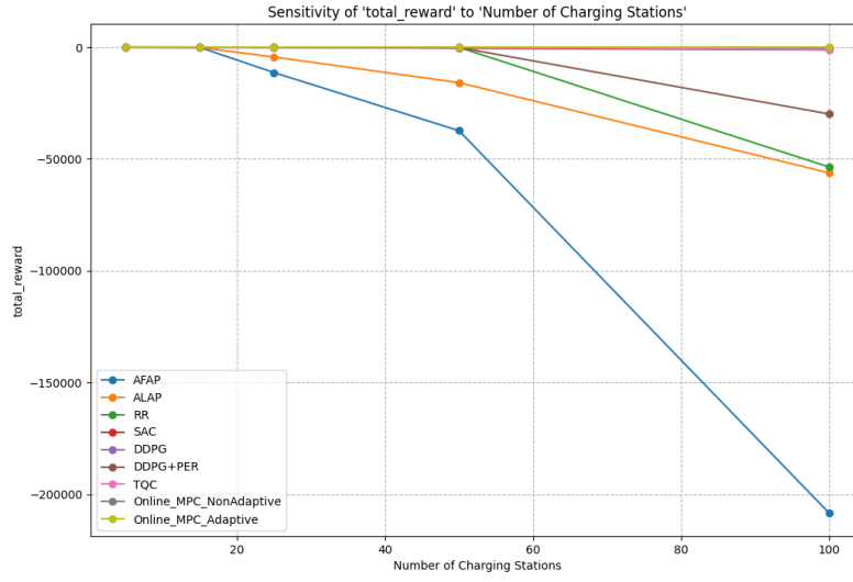
Figure 4.20: Sensitivity of Total Reward to the Number of Charging Stations.
