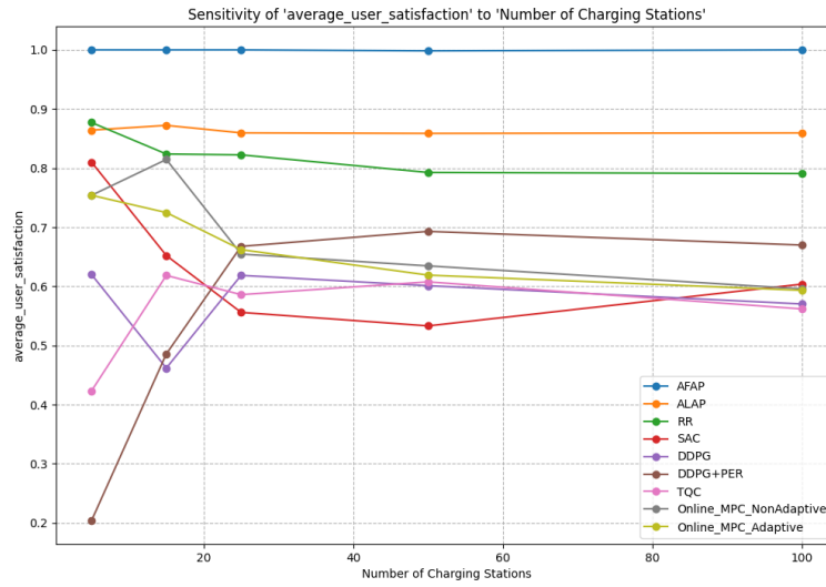
Figure 4.3: Sensitivity of Average User Satisfaction to the Number of Charging Stations.
