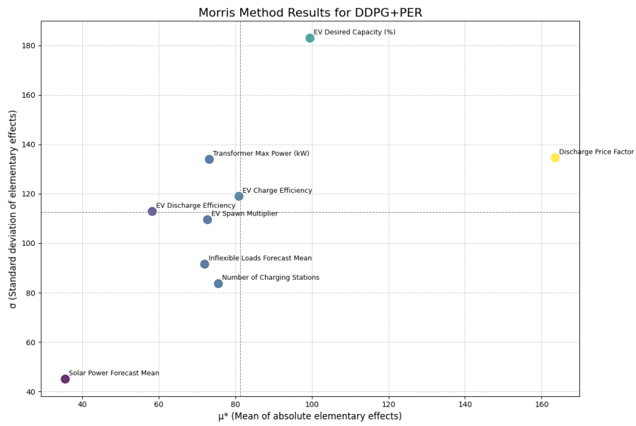
Figure 4.27: Morris method sensitivity plot for the DDPG+PER algorithm.
