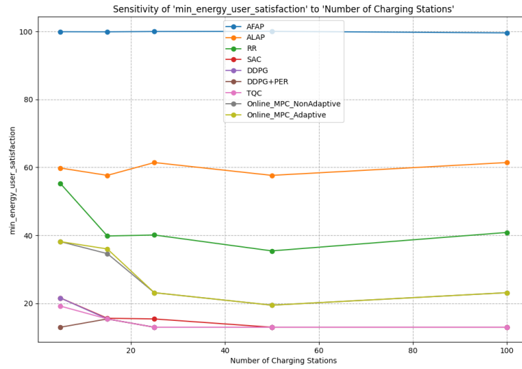
Figure 4.12: Sensitivity of Min Energy User Satisfaction to the Number of Charging Stations.
