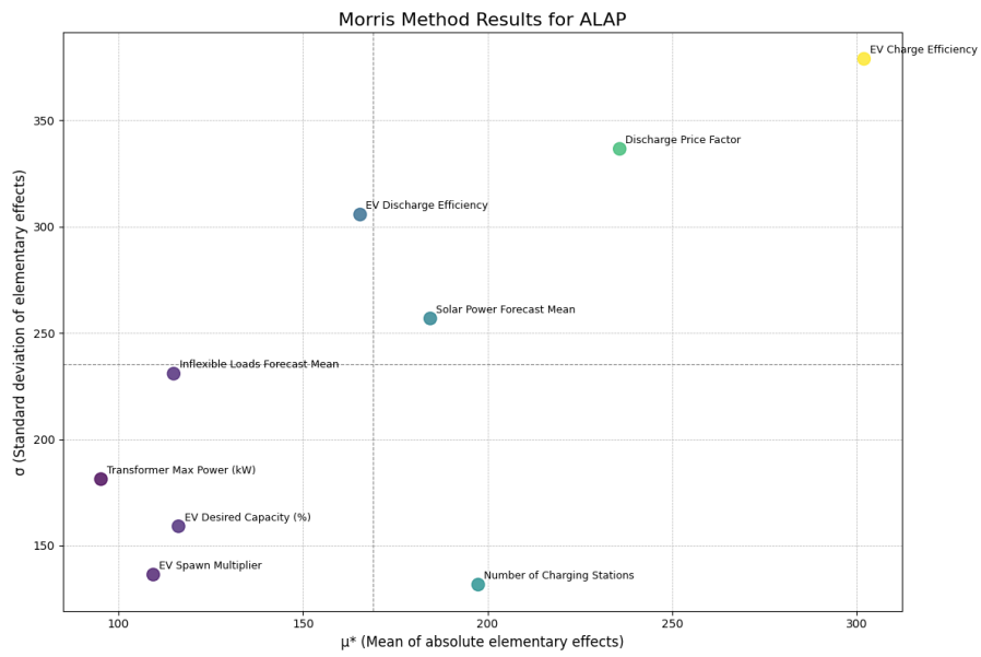
Figure 4.25: Morris method sensitivity plot for the ALAP algorithm.
