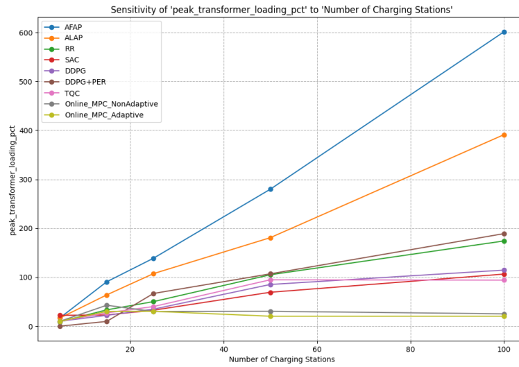
Figure 4.13: Sensitivity of Peak Transformer Loading Pct to the Number of Charging Stations.
