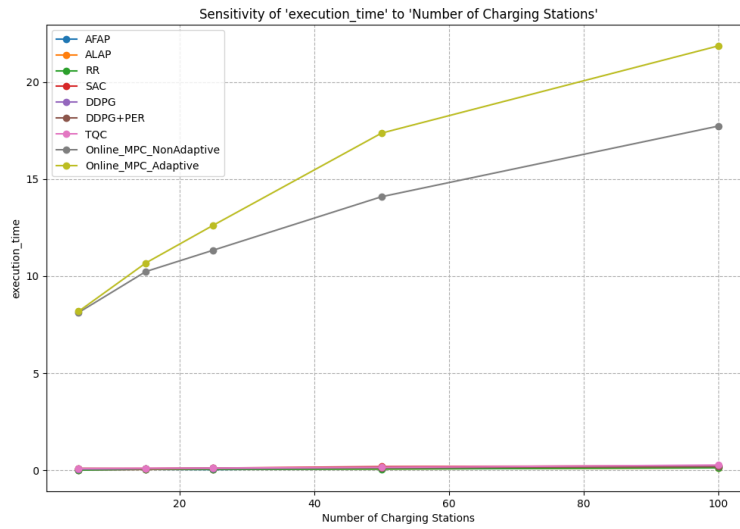
Figure 4.11: Sensitivity of Execution Time to the Number of Charging Stations.
