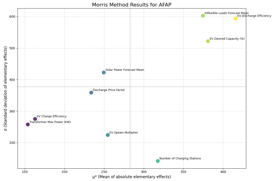
Figure 4.24: Morris method sensitivity plot for the AFAP algorithm.
