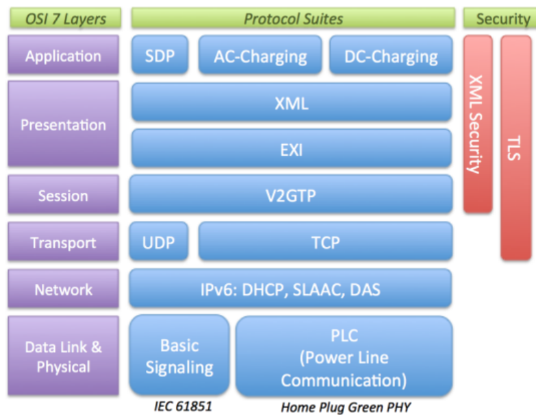
Figure 2.4: The protocol stack of ISO/IEC 15118 [43]
