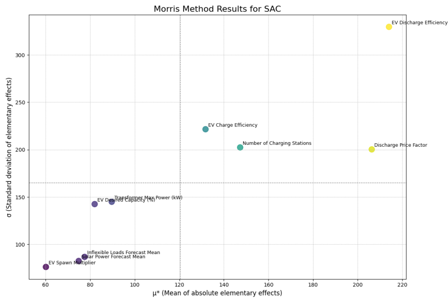
Figure 4.31: Morris method sensitivity plot for the SAC algorithm.
