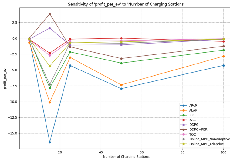
Figure 4.15: Sensitivity of Profit Per Ev to the Number of Charging Stations.
