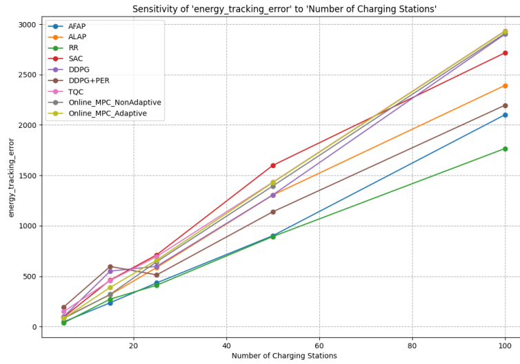
Figure 4.9: Sensitivity of Energy Tracking Error to the Number of Charging Stations.
