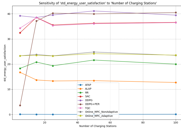
Figure 4.16: Sensitivity of Std Energy User Satisfaction to the Number of Charging Stations.
