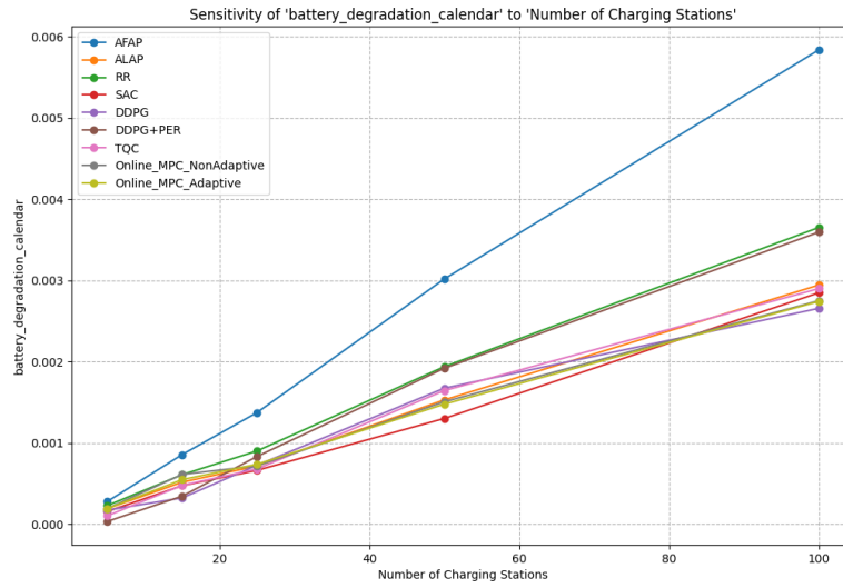
Figure 4.4: Sensitivity of Battery Degradation Calendar to the Number of Charging Stations.
