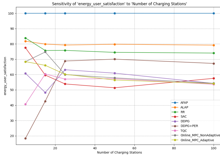
Figure 4.10: Sensitivity of Energy User Satisfaction to the Number of Charging Stations.
