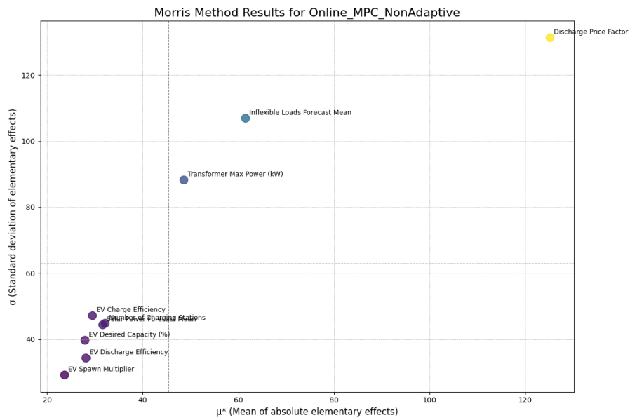
Figure 4.29: Morris method sensitivity plot for the Online MPC NonAdaptive algorithm.
