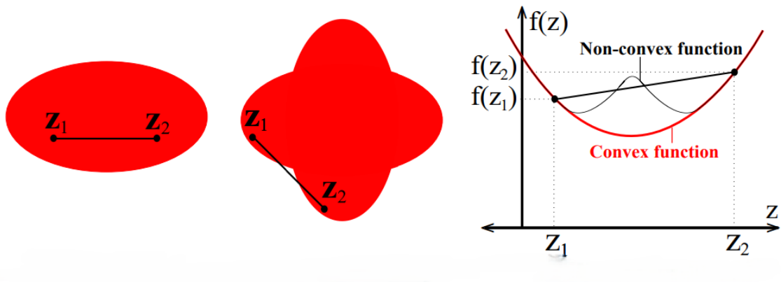
Figure 2.13: On the left, a convex set; in the middle, a non-convex set; on the right, a convex function.
