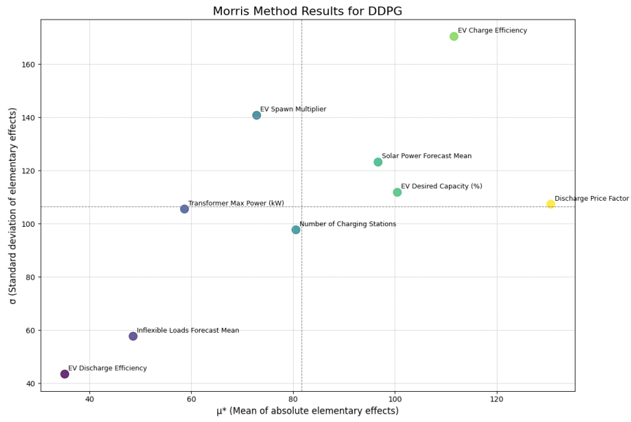
Figure 4.26: Morris method sensitivity plot for the DDPG algorithm.
