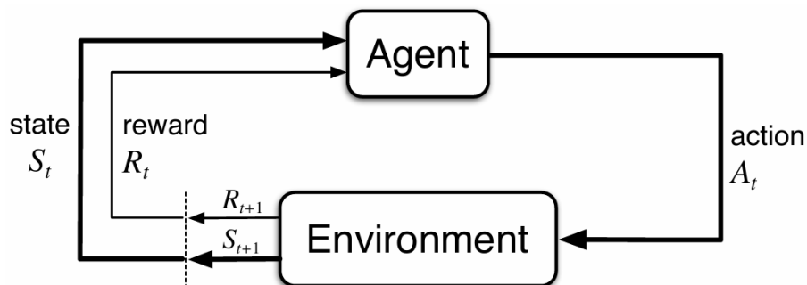
Figure 2.7: The agent-environment interaction loop in reinforcement learning [45].
