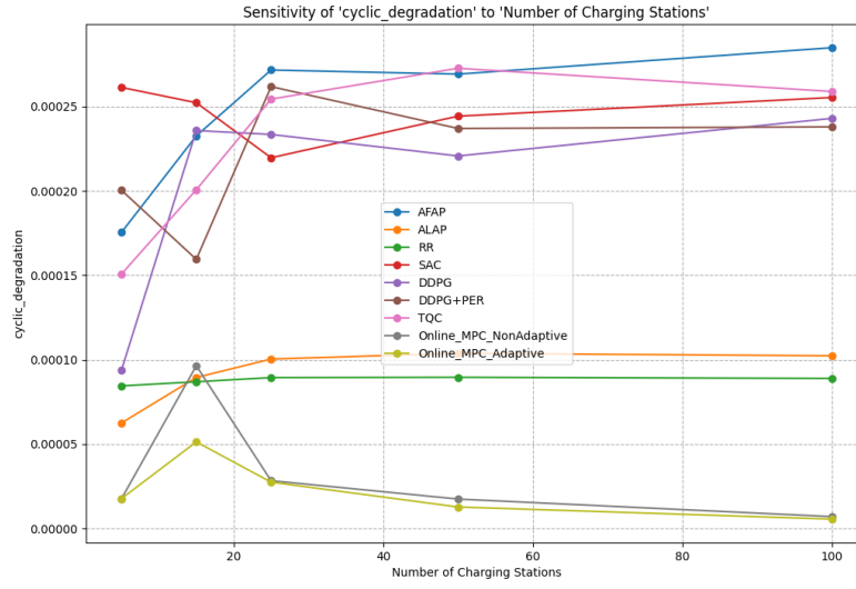
Figure 4.8: Sensitivity of Cyclic Degradation to the Number of Charging Stations.
