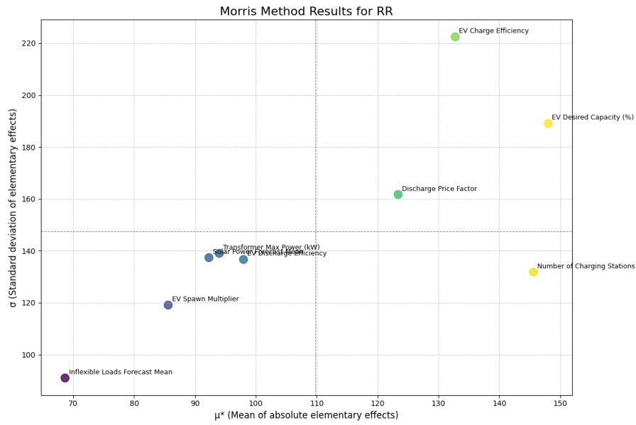
Figure 4.30: Morris method sensitivity plot for the RR algorithm.
