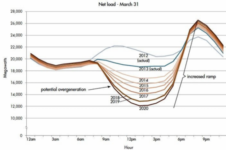
Figure 2.3: The "Duck Curve" illustrating the evolution of net load on the California grid.
