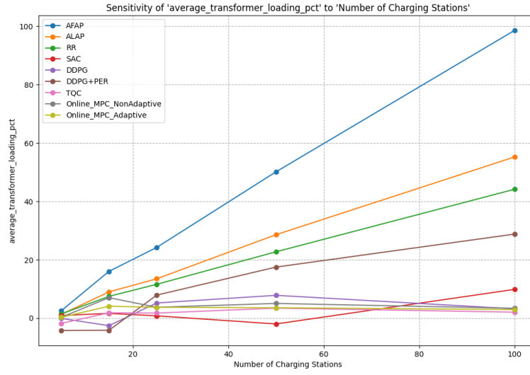
Figure 4.2: Sensitivity of Average Transformer Loading Pct to the Number of Charging Stations.
