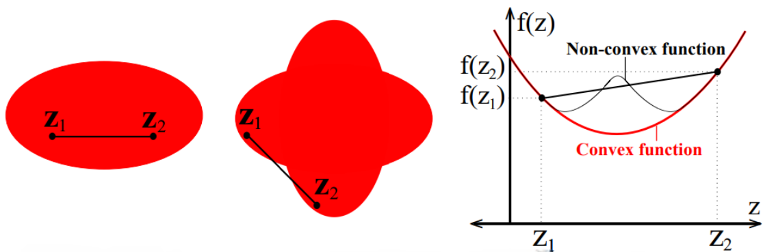
Figure 2.14: On the left, a convex set; in the middle, a non-convex set; on the right, a convex function.
