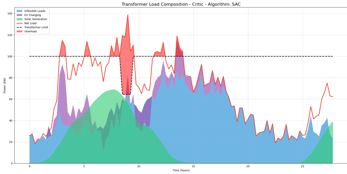
Figure 3.17: SAC
