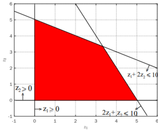
Figure 2.13: Constraint set (Polyhedron)
