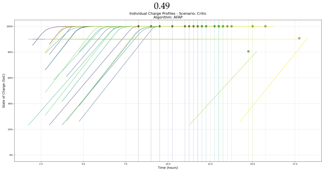
Figure 3.23: AFAP
