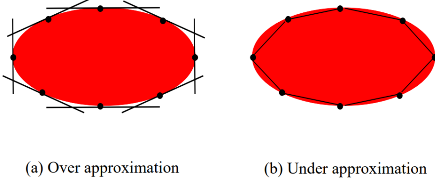
Figure 2.15: Approximating a convex set with a polytope
