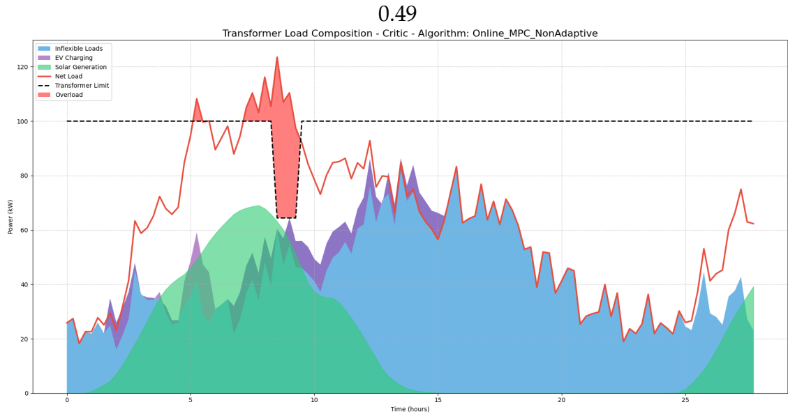
Figure 3.14: MPC Non-Adaptive
