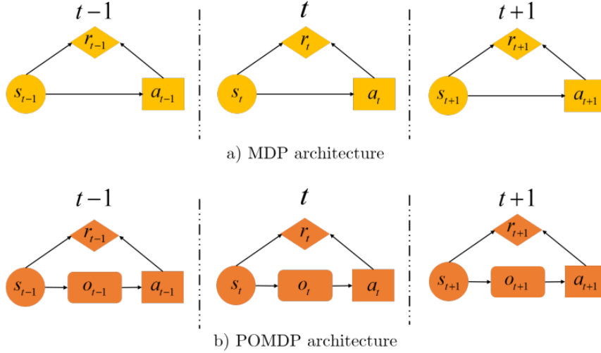
Figure 2.9: Differences between POMDP and MDP [38].
