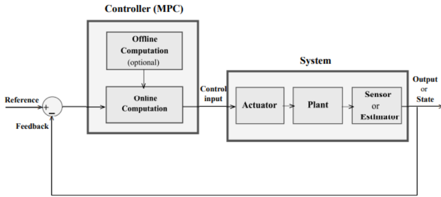
Figure 2.12: MPC: Block diagram
