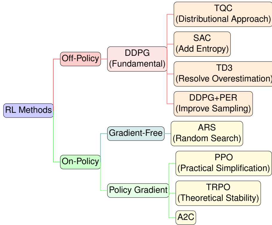
Figure 2.11: Hierarchical classification of Reinforcement Learning methods.
