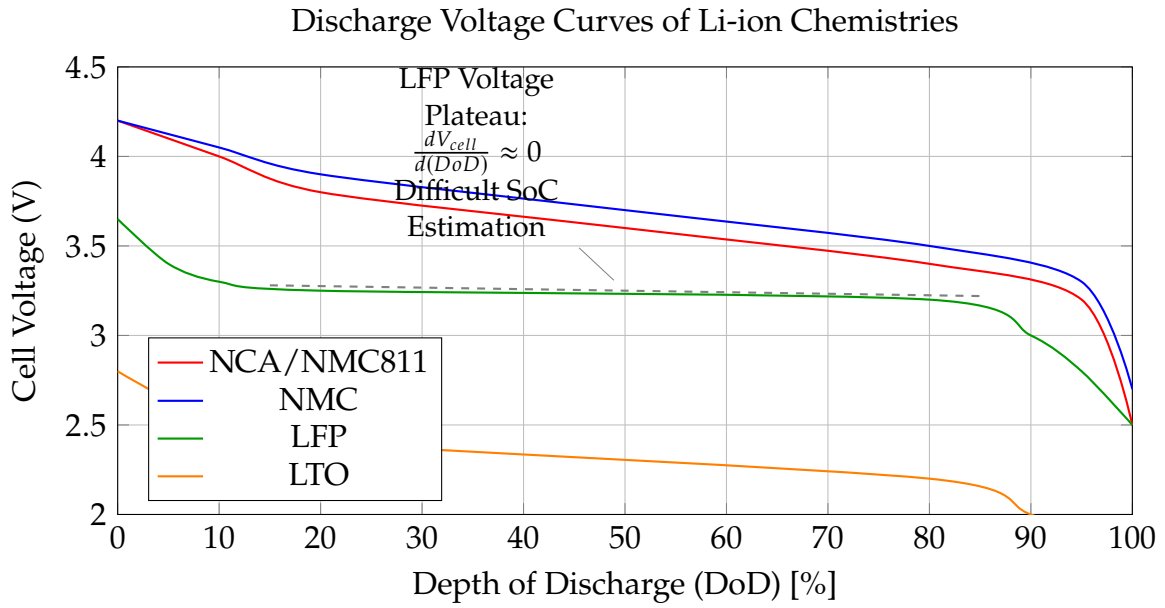
Figure 2.17: Typical discharge voltage curves for various lithium-ion chemistries. The extremely flat profile of LFP makes accurate SoC estimation challenging based on voltage alone, necessitating more complex estimation techniques like Coulomb counting and periodic recalibration.
