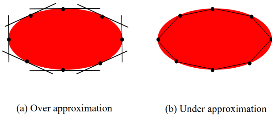
Figure 2.14: Approximating a convex set with a polytope
