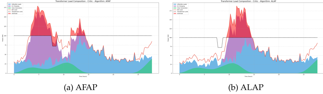
Figure 3.11: Grid load for heuristic algorithms. Both AFAP and ALAP show significant and prolonged periods of transformer overload, as they do not coordinate charging to respect grid limits.
