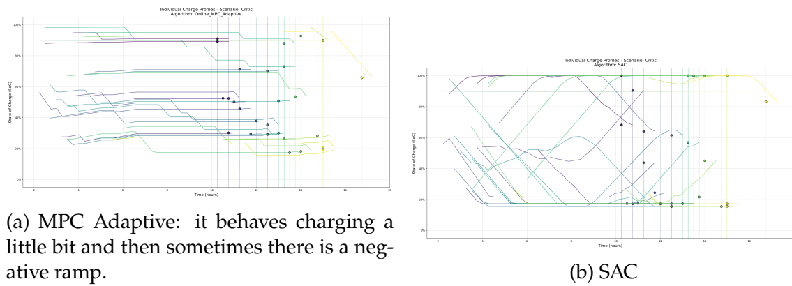
Figure 3.16: The SAC tends to fully charge some EVs while leaving others partially charged, focusing instead on using certain vehicles to maximize profit.
