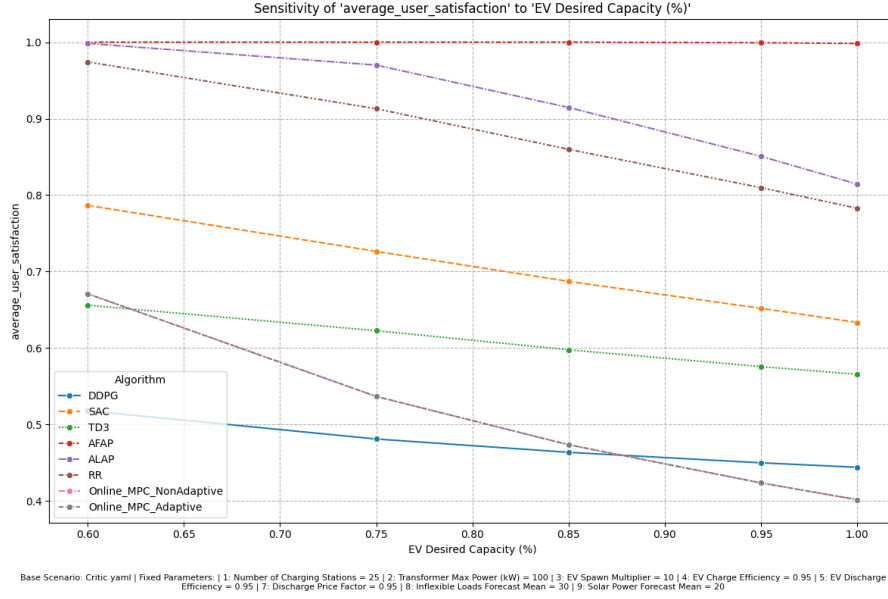
Figure 4.6: Impact of EV Desired Capacity on Average User Satisfaction.
