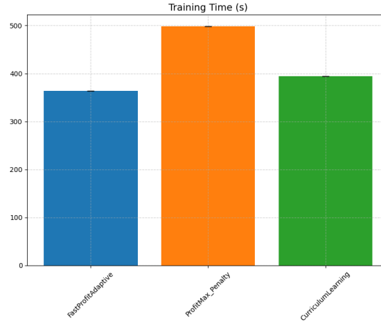
Figure 4.7: Training time performance comparison between the original reward function ( ProfitMax_Penalty ) and the new adaptive function ( FastProfitAdaptive ), with and without Curriculum Learning.
