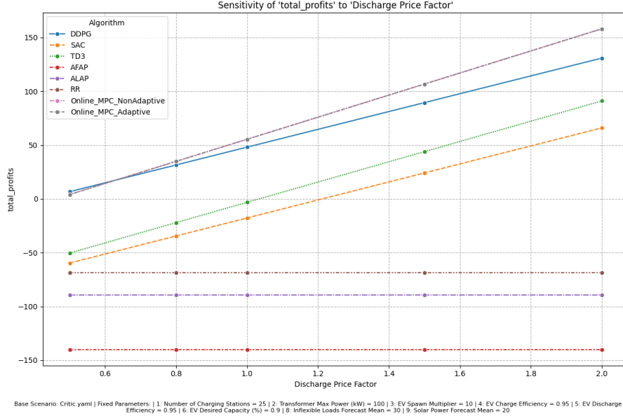
Figure 4.3: Impact of Discharge Price Factor on Total Profits for various algorithms.
