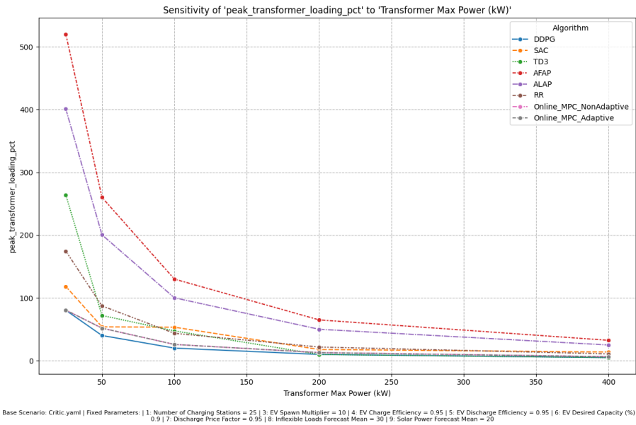
Figure 4.5: Impact of Transformer Max Power on Peak Transformer Loading.
