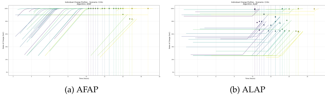
Figure 3.15: Individual EV profiles for heuristic algorithms. AFAP charges immediately upon arrival, while ALAP waits until the last possible moment. Neither strategy responds to price signals.
