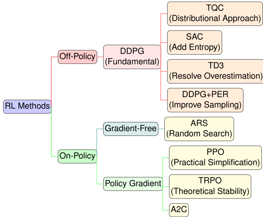
Figure 2.12: Hierarchical classification of Reinforcement Learning methods.
