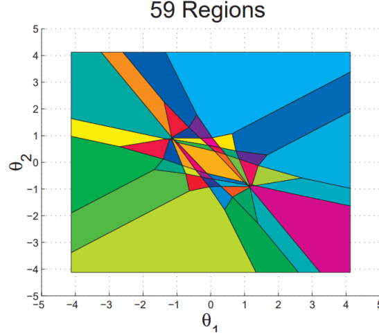
Figure 2.17: Example of a structure of a polyhedral region by Alberto Bemporad and Carlo Filippi
