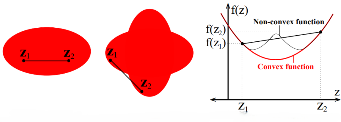
Figure 2.15: On the left, a convex set; in the middle, a non-convex set; on the right, a convex function.
