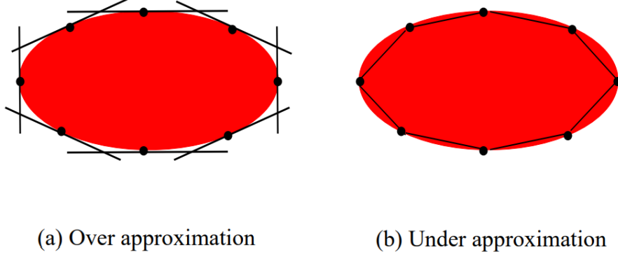
Figure 2.16: Approximating a convex set with a polytope
