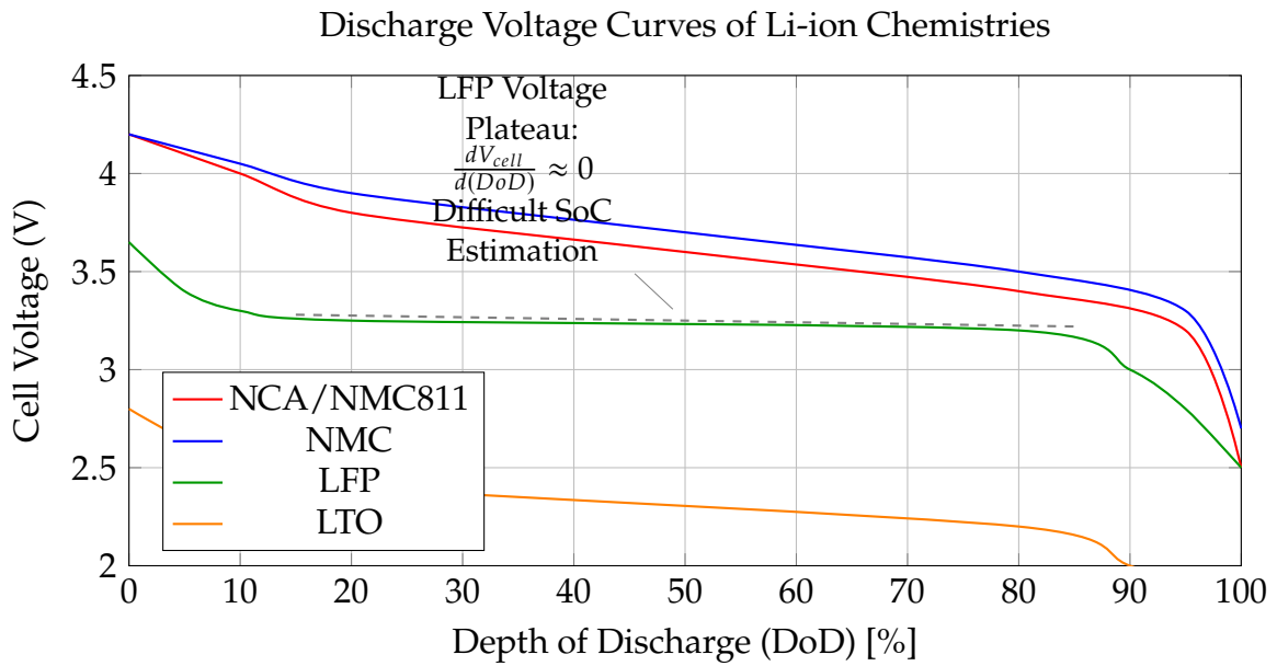
Figure 2.18: Typical discharge voltage curves for various lithium-ion chemistries. The extremely flat profile of LFP makes accurate SoC estimation challenging based on voltage alone, necessitating more complex estimation techniques like Coulomb counting and periodic recalibration.
