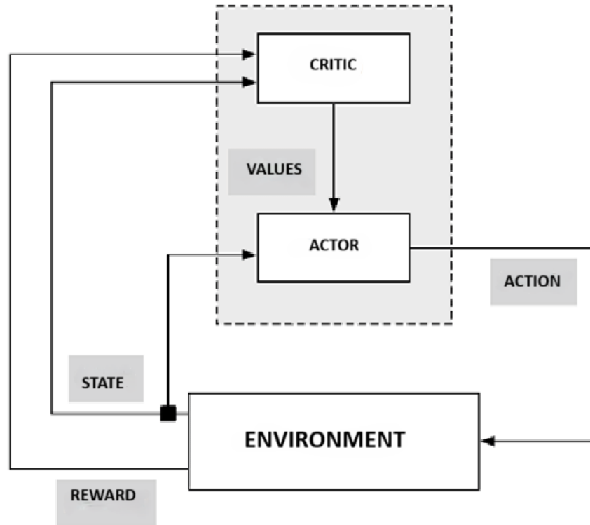
Figure 2.10: The Actor Critic scheme
