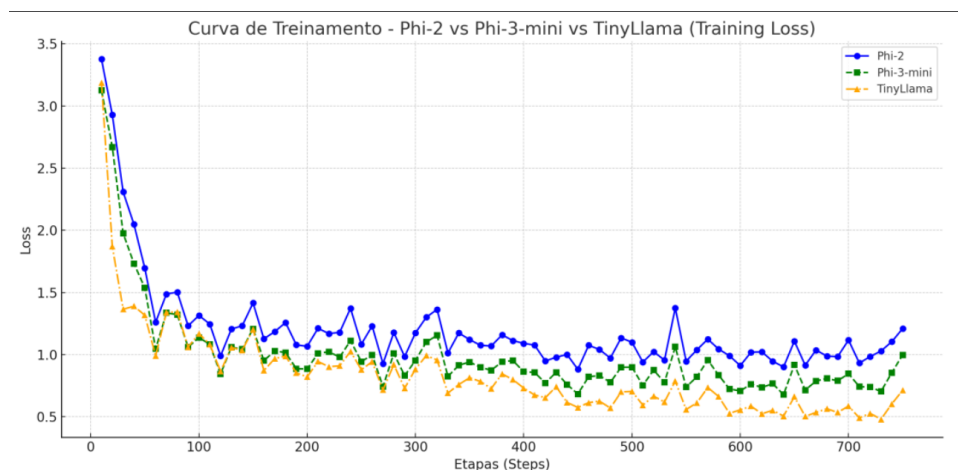
Figura 1. Curva de Loss – Phi-2 vs Phi-3-mini vs TinyLlama
