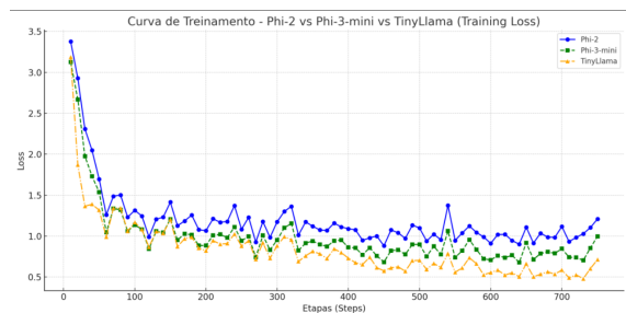
Fig. 2. Curva de Loss – Phi-2 vs Phi-3-mini vs TinyLlama
