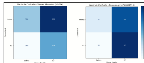
Fig. 8. Confusion Matrix – VGG16.
