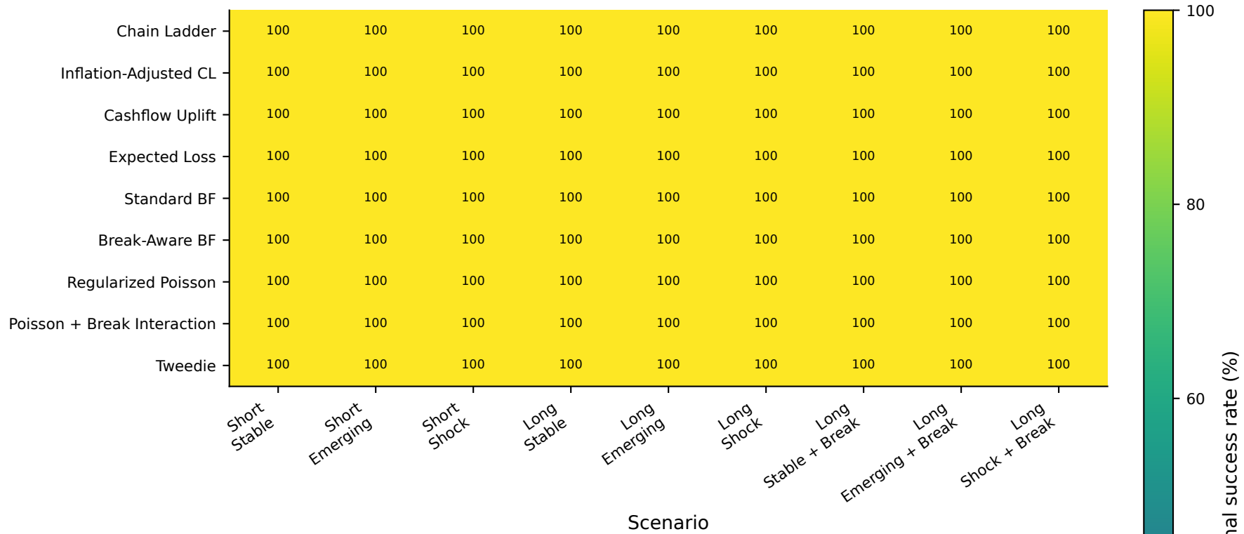
Figure 2. Baseline model estimation success
