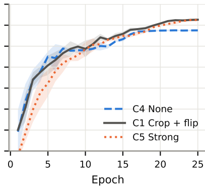
Augmentation
