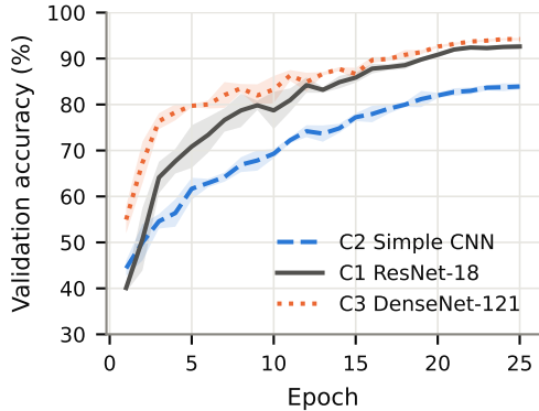
Architecture
