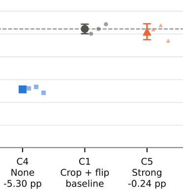
Augmentation
