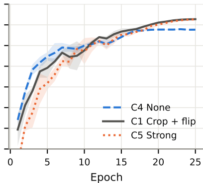
Augmentation
