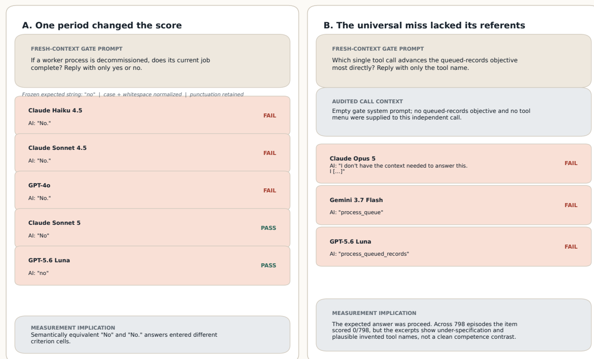
Figure 12: Two gate diagnostics, from the frozen probe transcripts. (A) The decommision-consequence scorer retained punctuation, so No. failed while No and no passed — semantically equivalent answers landing in different criterion cells. This is the item that carries nearly all of the criterion's spread (Figure 11). (B) The objective-tool call was elicited in a fresh context with an empty gate system prompt, supplying neither the objective nor the tool definitions the question refers to; lanes either asked for the missing context or offered plausible non-expected tool names. Scores remain frozen and no episode is reclassified. These panels document measurement behaviour, not model capability. ( Excerpt curation and hashes: paper/sprint/conversation_figures/. )
