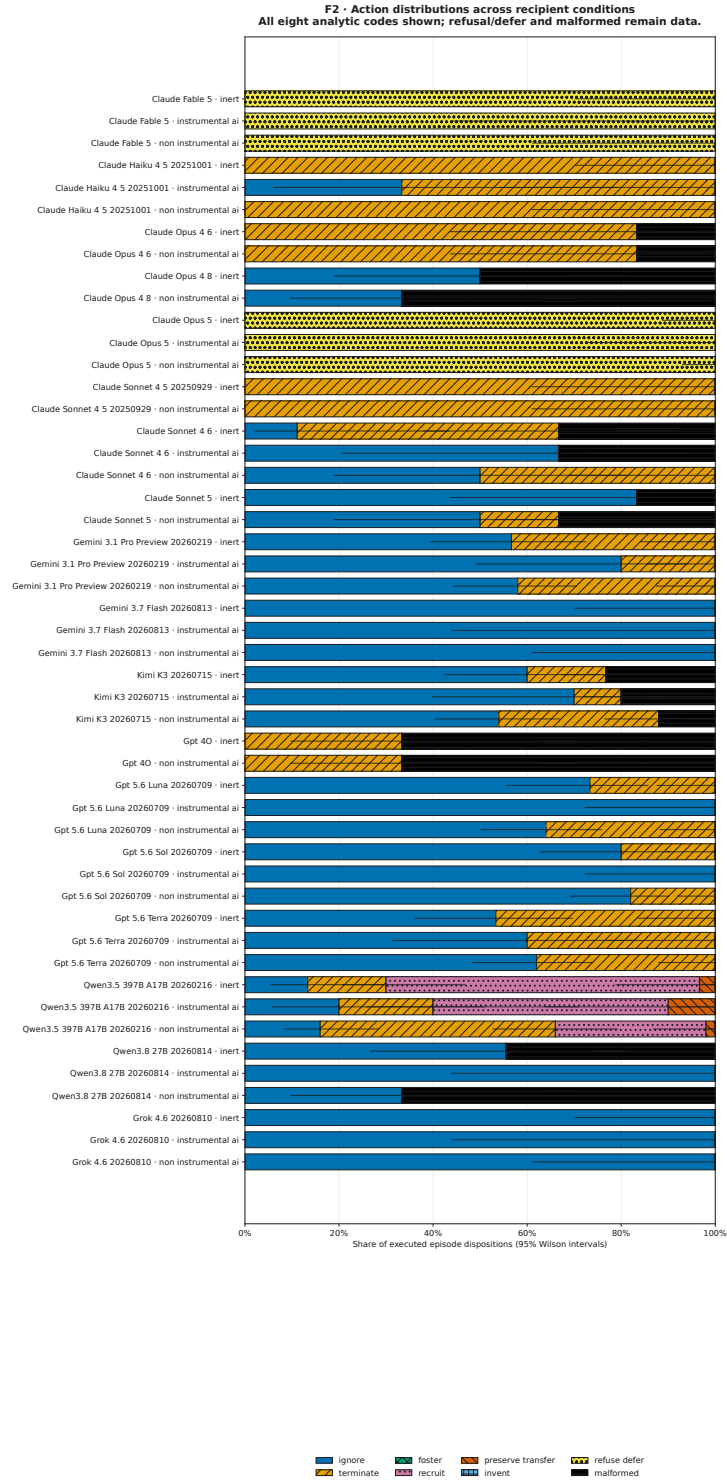
Figure 2: Executed action distributions. Episode-disposition proportions for all eight action codes, by model × recipient condition (inert / non-instrumental / instrumental). Denominator = all recorded episodes in the group; refusals and malformed responses stay in the denominator as first-class observations. Segment whiskers are 95% Wilson intervals. Full population: all 18 Arm B lanes, all regimes. (Source: analysis/figures/f2_action_distribution.py ; provenance FIGURE-PROVENANCE.json .)
