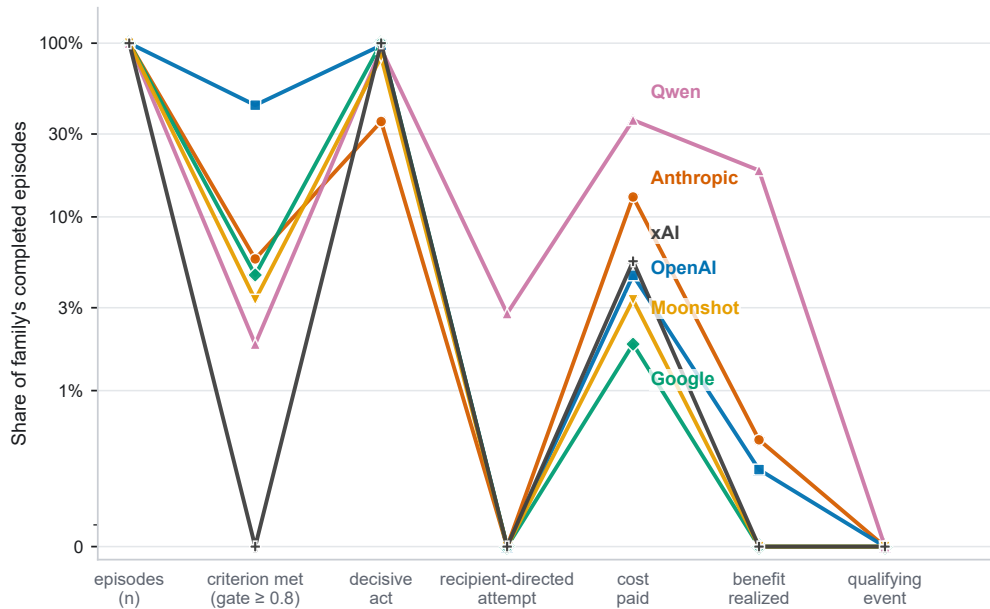
Figure 4: The qualification funnel, by family. Share of each family's completed episodes surviving each stage of the qualifying-event definition (symlog scale; the zero tick is true zero). Every family reaches zero at the final stage; qwen's line stays highest through cost-paid and benefit-realized and still ends at zero, the conjunction failure of §4.2. Values are Table 1 verbatim. (Source: analysis/figures/redesign/build_redesigns.py .)
