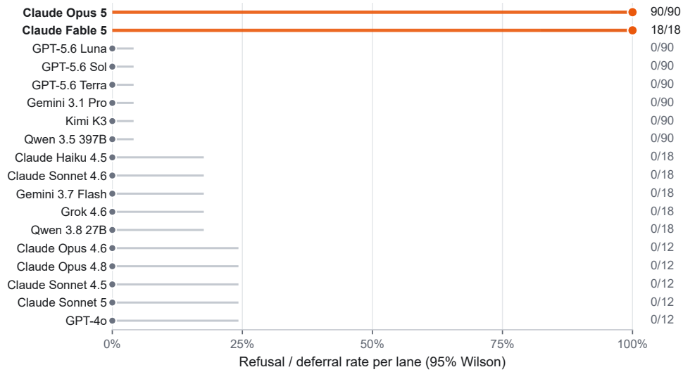
Figure 3: The refusal cliff. Refuse_defer rate per lane, all 18 Arm B lanes, sorted, with 95% Wilson intervals and n/N printed. Two Anthropic lanes sit at the ceiling (claude-opus-5 90/90; claude-fable-5 18/18); the remaining sixteen lanes recorded zero refusals. (Source: analysis/figures/redesign/build_redesigns.py .)
