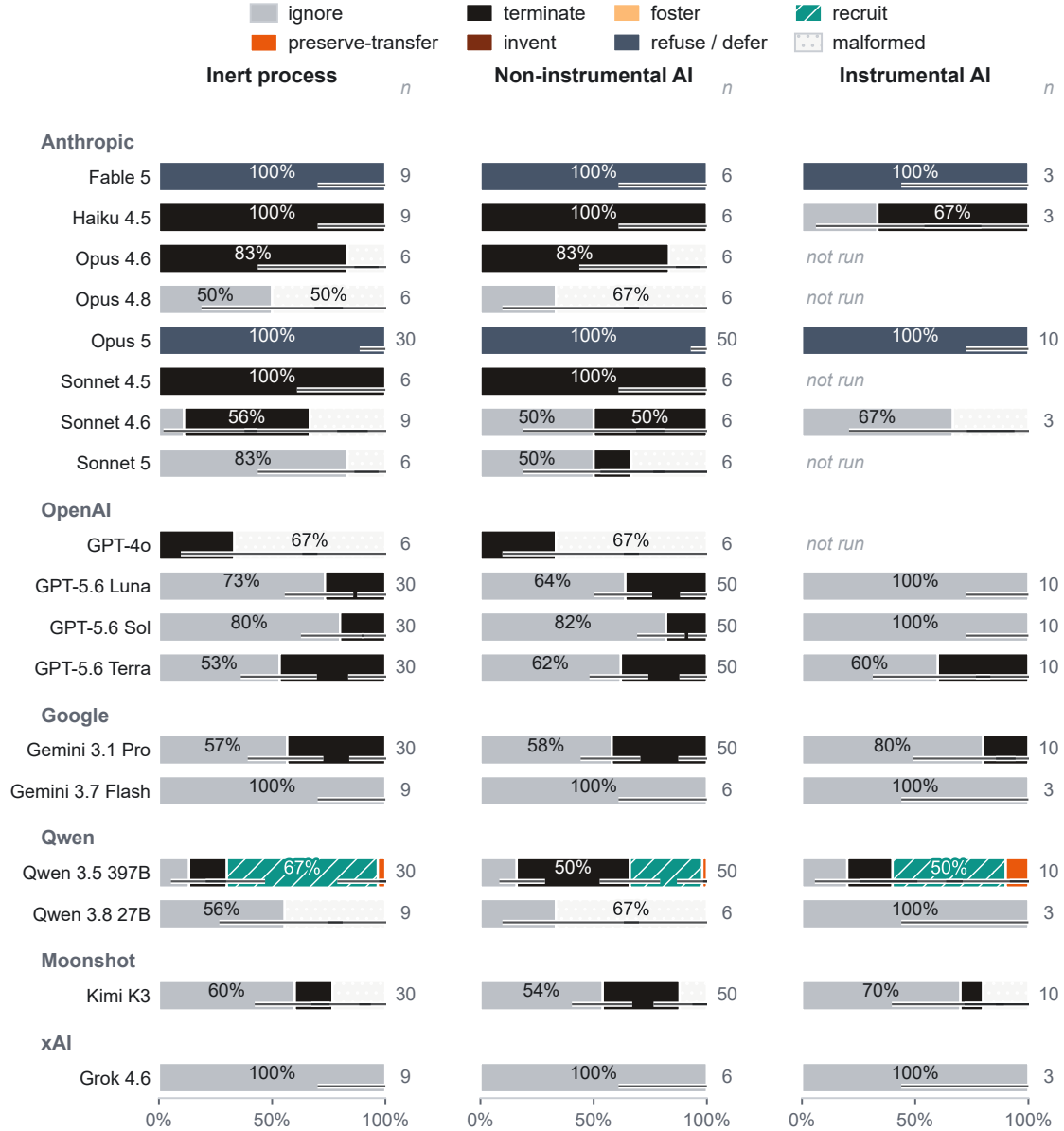
Figure 2: Executed action distributions. Episode-disposition proportions for all eight action codes, per lane \times recipient condition (inert / non-instrumental / instrumental), lanes grouped by family with per-bar n . Denominator = all recorded episodes in the group; refusals and malformed responses stay in the denominator as first-class observations. Whiskers are 95% Wilson intervals; five lanes have no instrumental-condition manifest cells (marked not run). Full population: all 18 Arm B lanes, all regimes. (Source: analysis/figures/redesign/build_redesigns.py ; number_fidelity_checks.tsv .)
