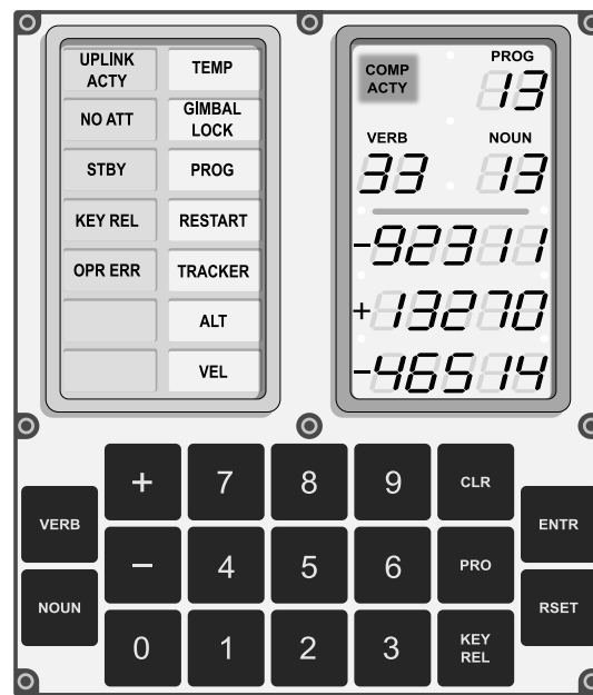
Figure 2.2: DSKY interface diagram by Oona Räisänen
