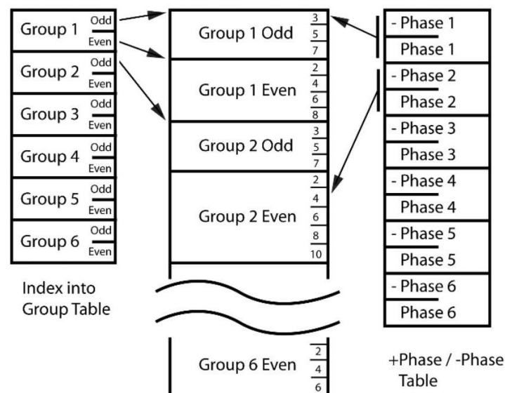
Figure 3.1: Restart and Phase Tables
