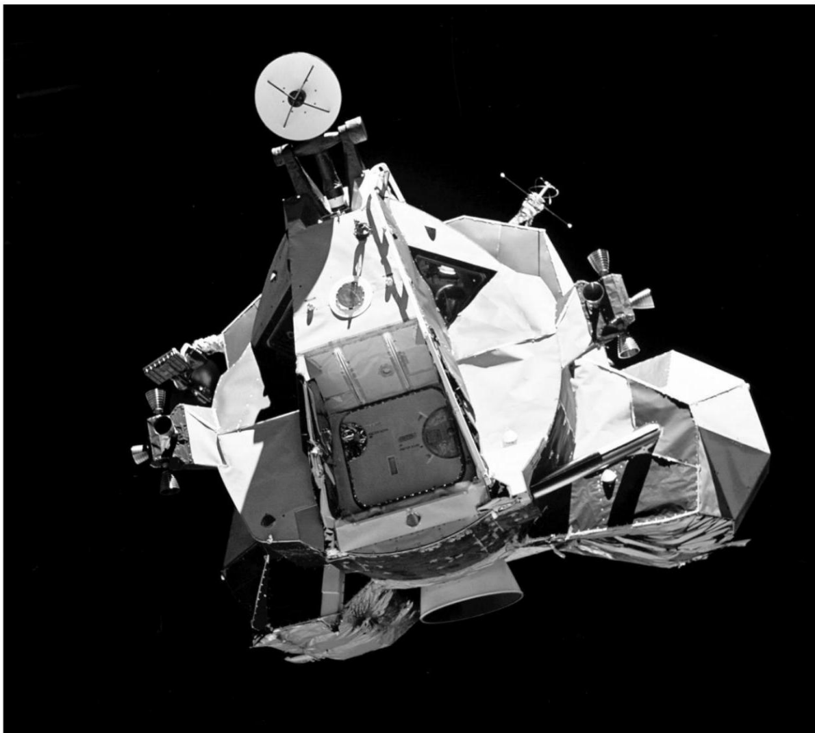
Figure 43: LM rendezvous radar at top of ascent stage electronics have not failed. A problem in these electronics will not cause a program alarm or terminate any active work, as to do so might cause a loss of data during the critical landing phase of the mission. Note that this is different from the “radar data not good” discrete, which is often due to an antenna positioning error and is not the result of a hardware failure. Although programs continue to run, the TRACKER warning light illuminates to warn the crew the radar
