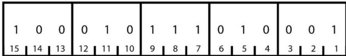
Figure 41: Data in INLINK register
