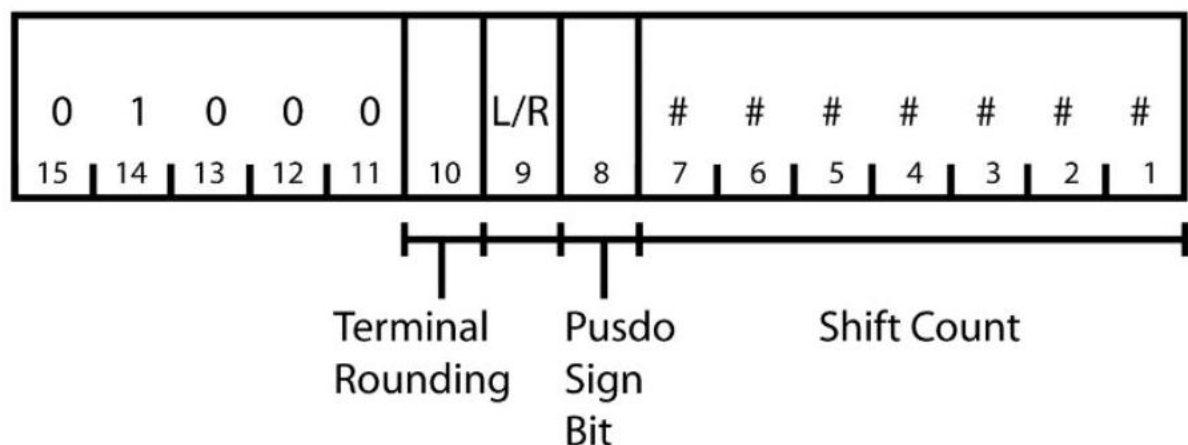
Figure 61: Long shift address word format
