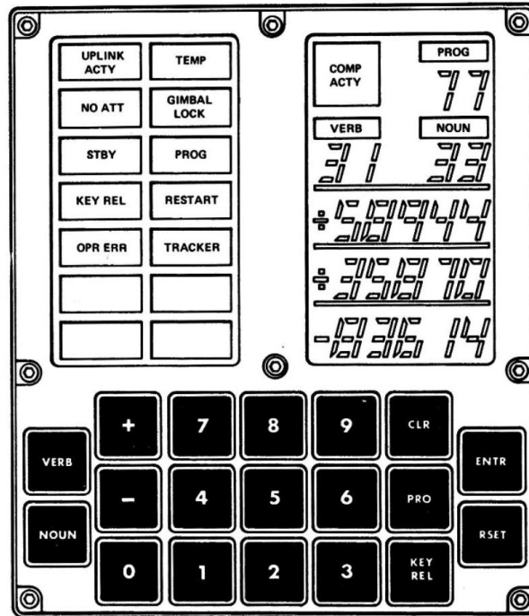
Figure 4.2: Diagram of the DSKY
