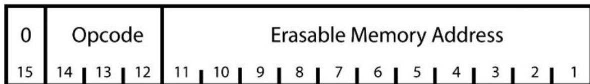
Figure 62: STORE instruction format
