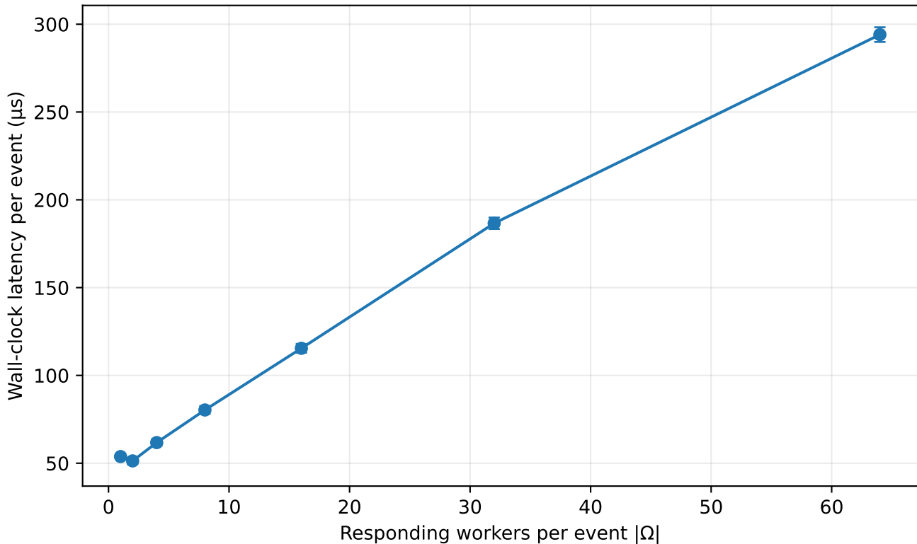
Cost grows with response sparsity, not total N
