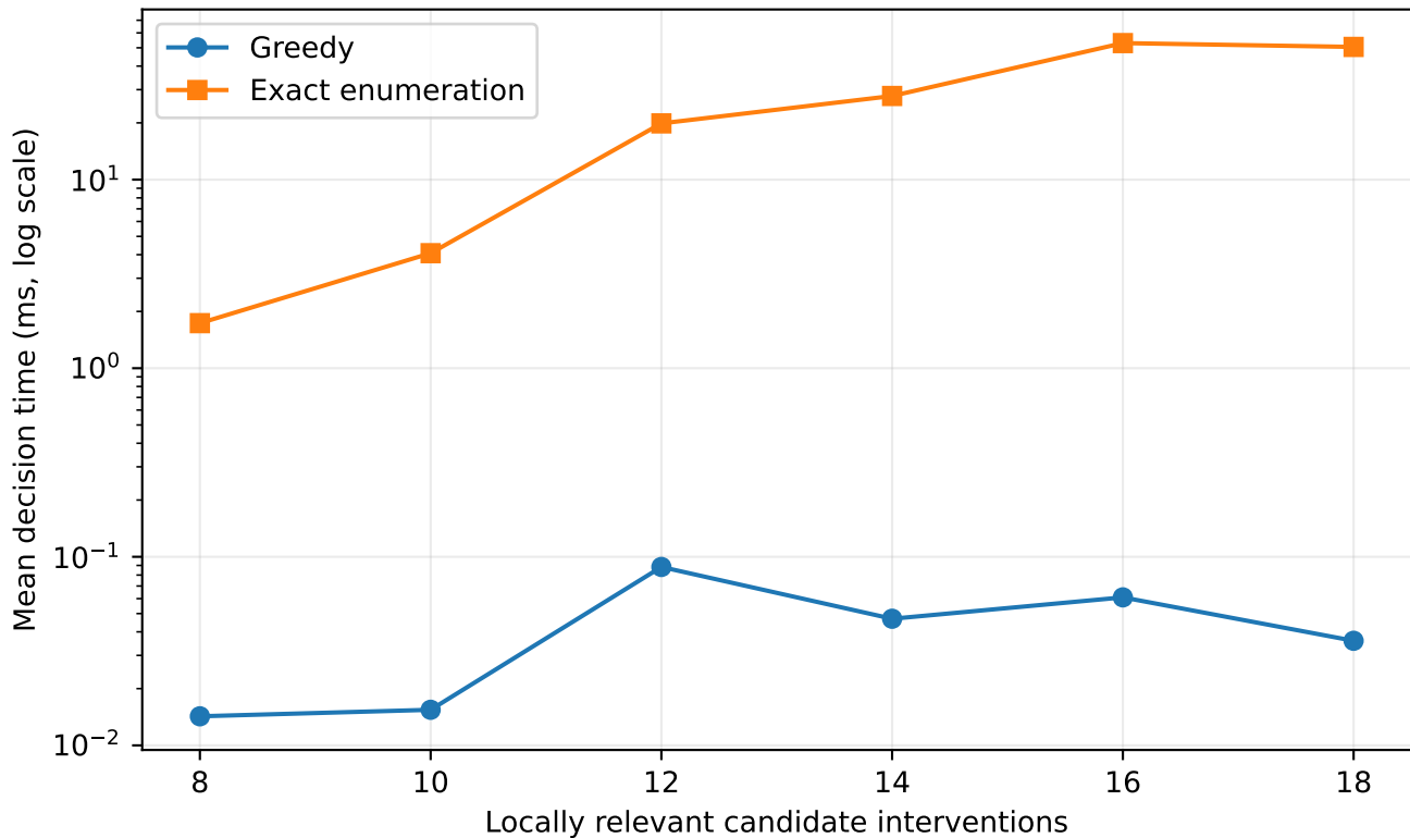
Greedy selection removes local combinatorial explosion
