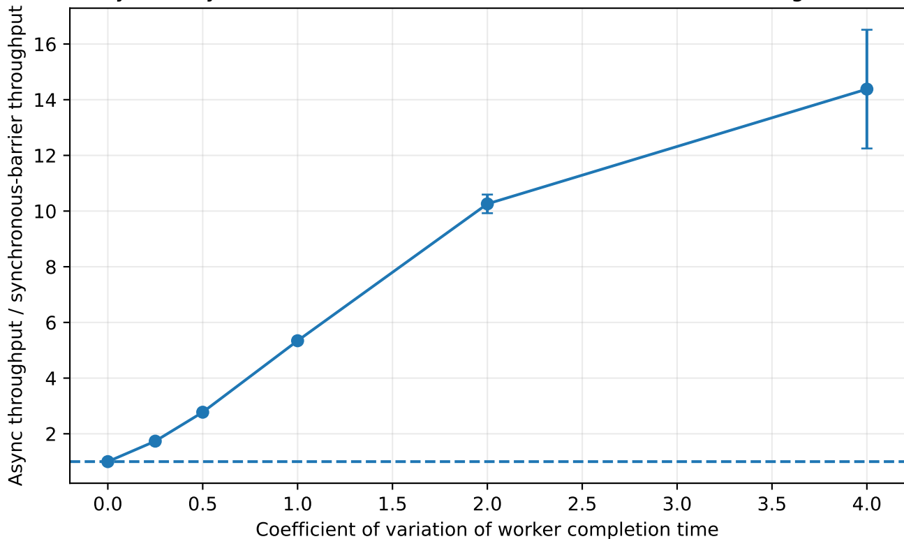
Asynchrony becomes valuable as worker times become heterogeneous
