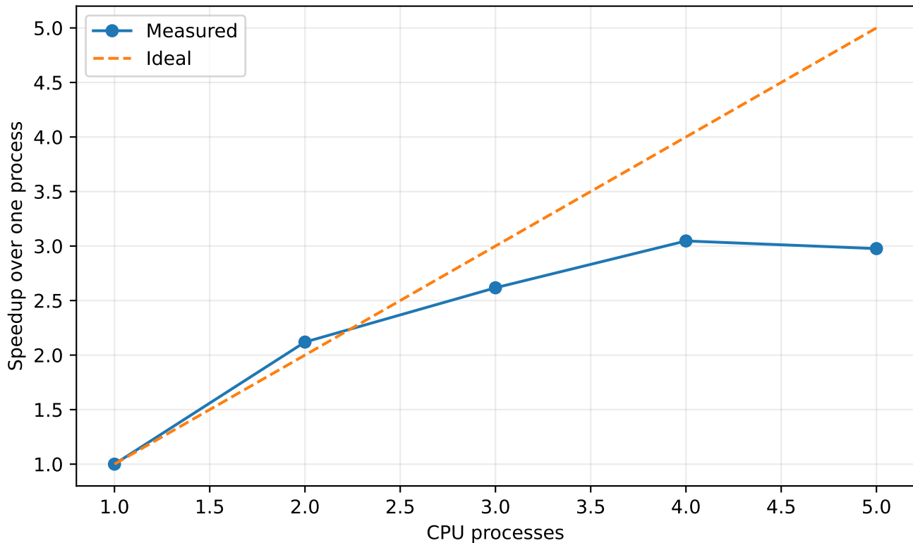
Parallel local candidate rollouts on CPU
